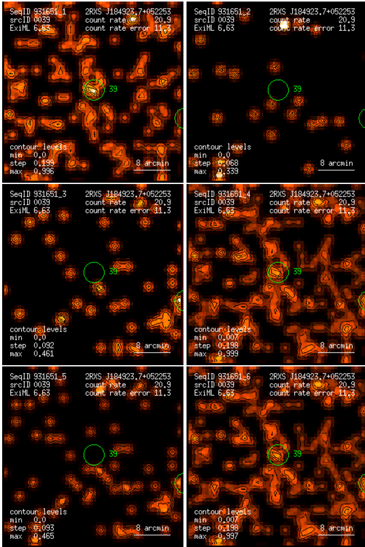
Figure 39: RASS 931651: detection 0039: band rate images, Gaussian filter: (1) PSPC channels 11 – 41, (2) 52 – 90, (3) 91 – 201, (4) 11 – 235, (5) 52 – 201, (6) 11 – 201. Broad band rates in counts/ks. Band rate contour levels in counts/ks/arcmin 2 .
