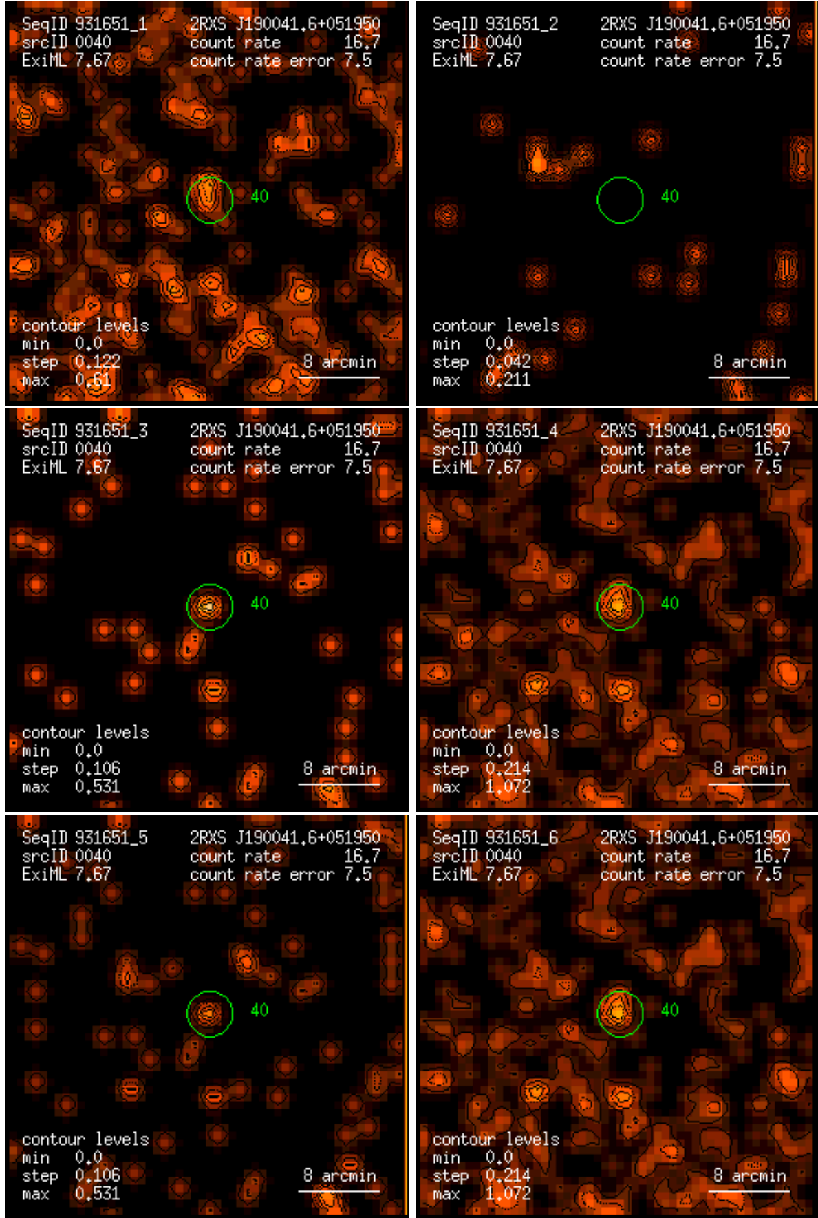
Figure 40: RASS 931651: detection 0040: band rate images, Gaussian filter: (1) PSPC channels 11 – 41, (2) 52 – 90, (3) 91 – 201, (4) 11 – 235, (5) 52 – 201, (6) 11 – 201. Broad band rates in counts/ks. Band rate contour levels in counts/ks/arcmin 2 .
