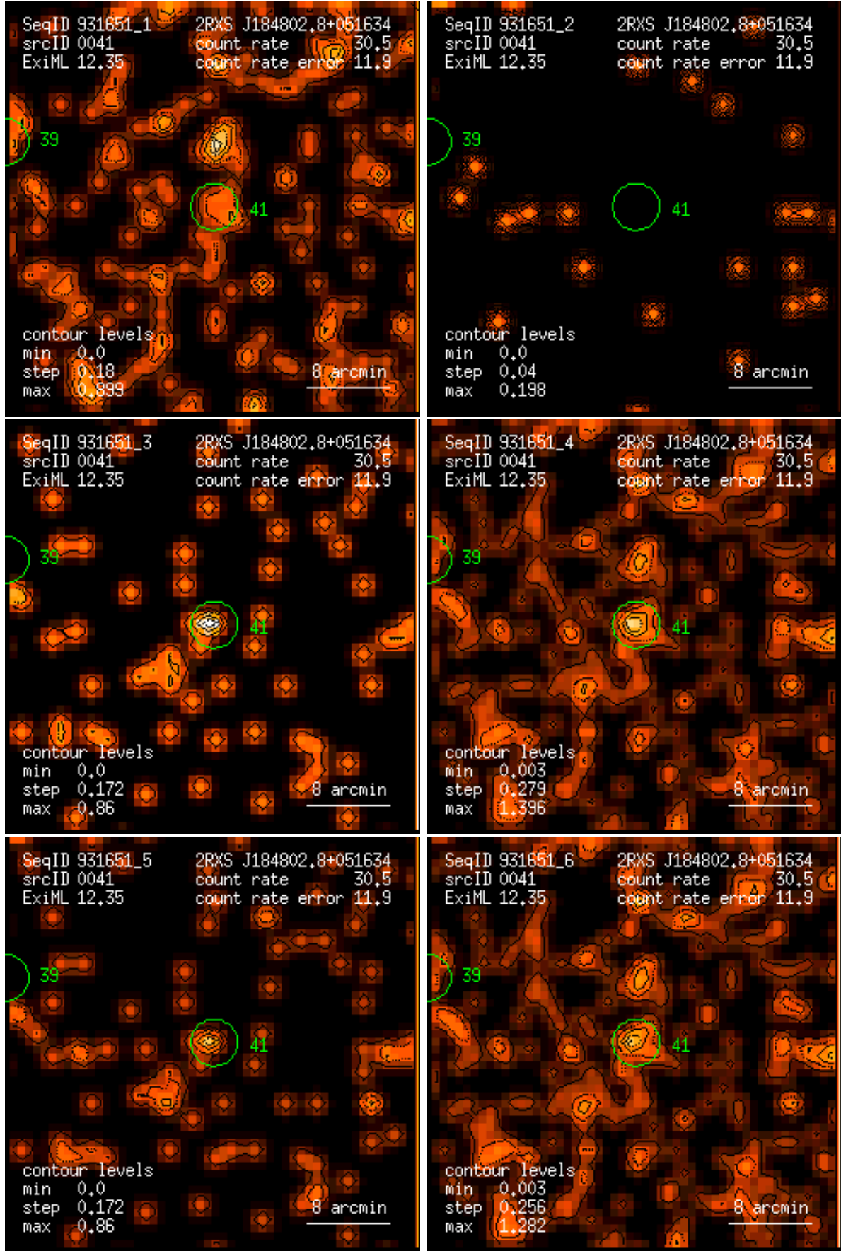
Figure 41: RASS 931651: detection 0041: band rate images, Gaussian filter: (1) PSPC channels 11 – 41, (2) 52 – 90, (3) 91 – 201, (4) 11 – 235, (5) 52 – 201, (6) 11 – 201. Broad band rates in counts/ks. Band rate contour levels in counts/ks/arcmin 2 .
