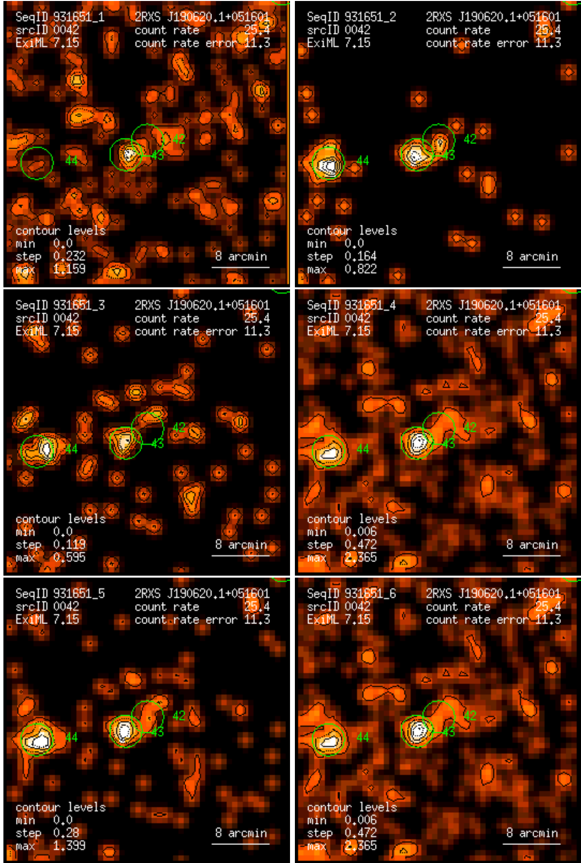
Figure 42: RASS 931651: detection 0042: band rate images, Gaussian filter: (1) PSPC channels 11 – 41, (2) 52 – 90, (3) 91 – 201, (4) 11 – 235, (5) 52 – 201, (6) 11 – 201. Broad band rates in counts/ks. Band rate contour levels in counts/ks/arcmin 2 .
