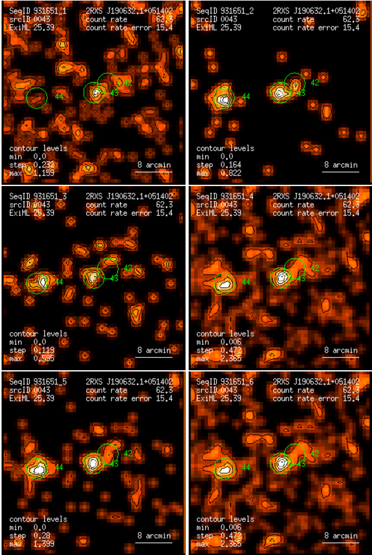
Figure 43: RASS 931651: detection 0043: band rate images, Gaussian filter: (1) PSPC channels 11 – 41, (2) 52 – 90, (3) 91 – 201, (4) 11 – 235, (5) 52 – 201, (6) 11 – 201. Broad band rates in counts/ks. Band rate contour levels in counts/ks/arcmin 2 .
