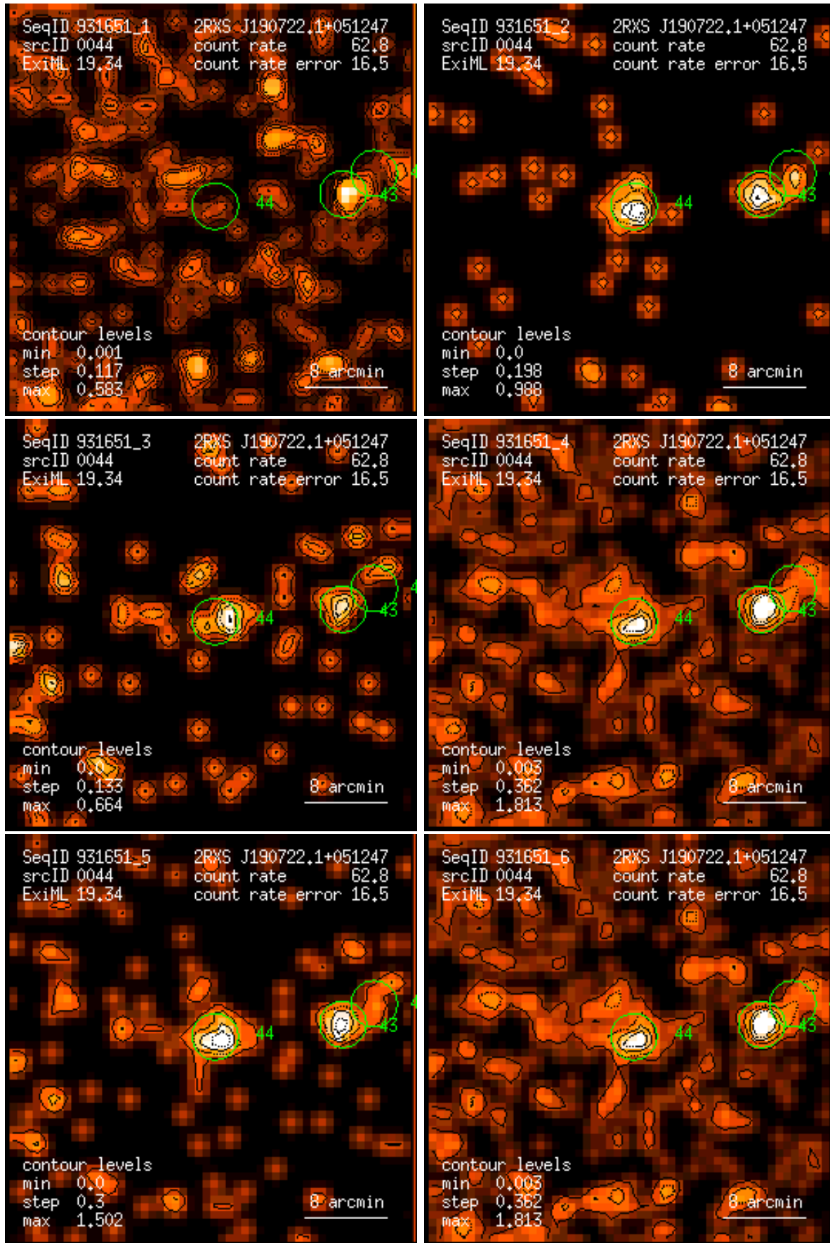
Figure 44: RASS 931651: detection 0044: band rate images, Gaussian filter: (1) PSPC channels 11 – 41, (2) 52 – 90, (3) 91 – 201, (4) 11 – 235, (5) 52 – 201, (6) 11 – 201. Broad band rates in counts/ks. Band rate contour levels in counts/ks/arcmin 2 .
