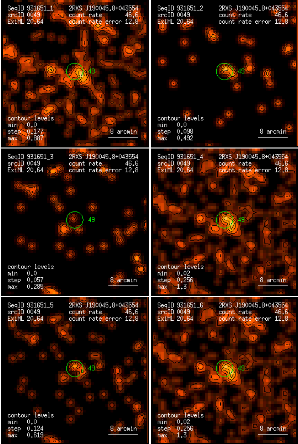
Figure 49: RASS 931651: detection 0049: band rate images, Gaussian filter: (1) PSPC channels 11 – 41, (2) 52 – 90, (3) 91 – 201, (4) 11 – 235, (5) 52 – 201, (6) 11 – 201. Broad band rates in counts/ks. Band rate contour levels in counts/ks/arcmin 2 .
