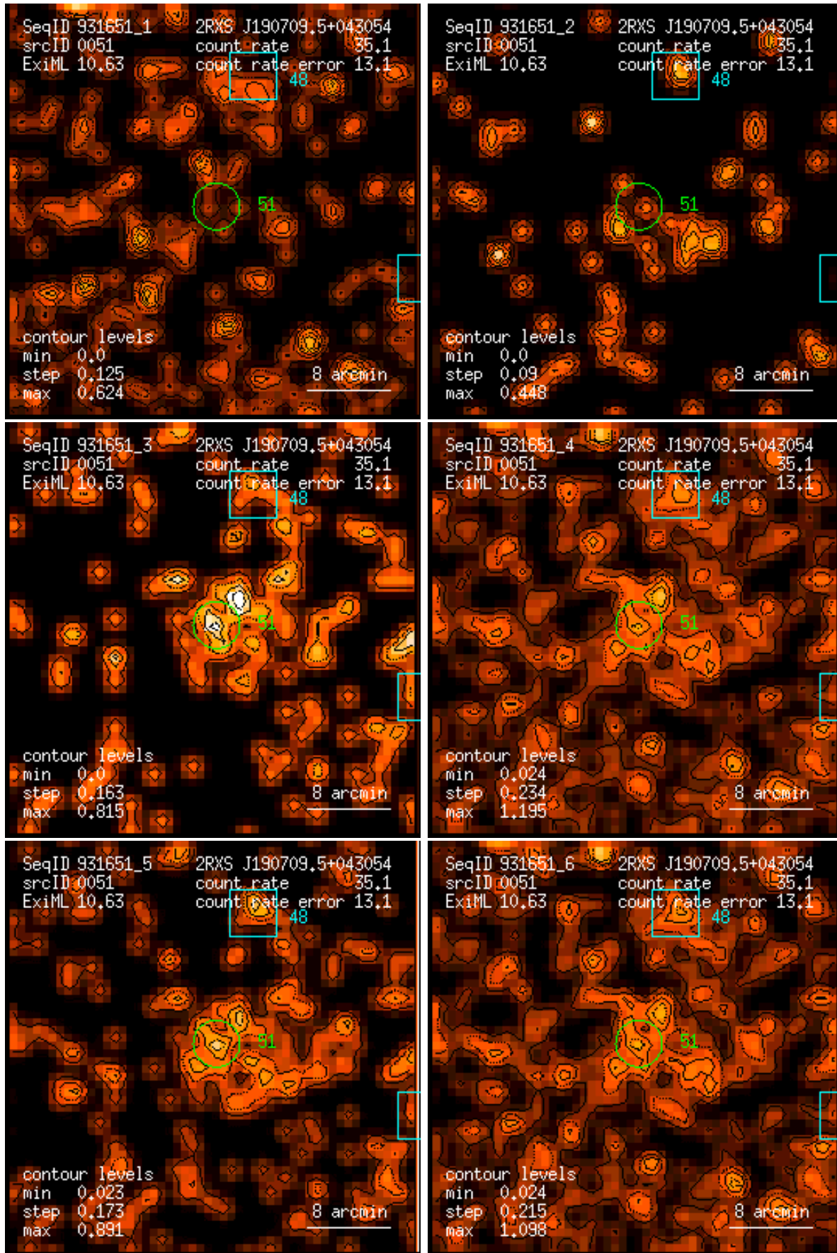
Figure 51: RASS 931651: detection 0051: band rate images, Gaussian filter: (1) PSPC channels 11 – 41, (2) 52 – 90, (3) 91 – 201, (4) 11 – 235, (5) 52 – 201, (6) 11 – 201. Broad band rates in counts/ks. Band rate contour levels in counts/ks/arcmin 2 .
