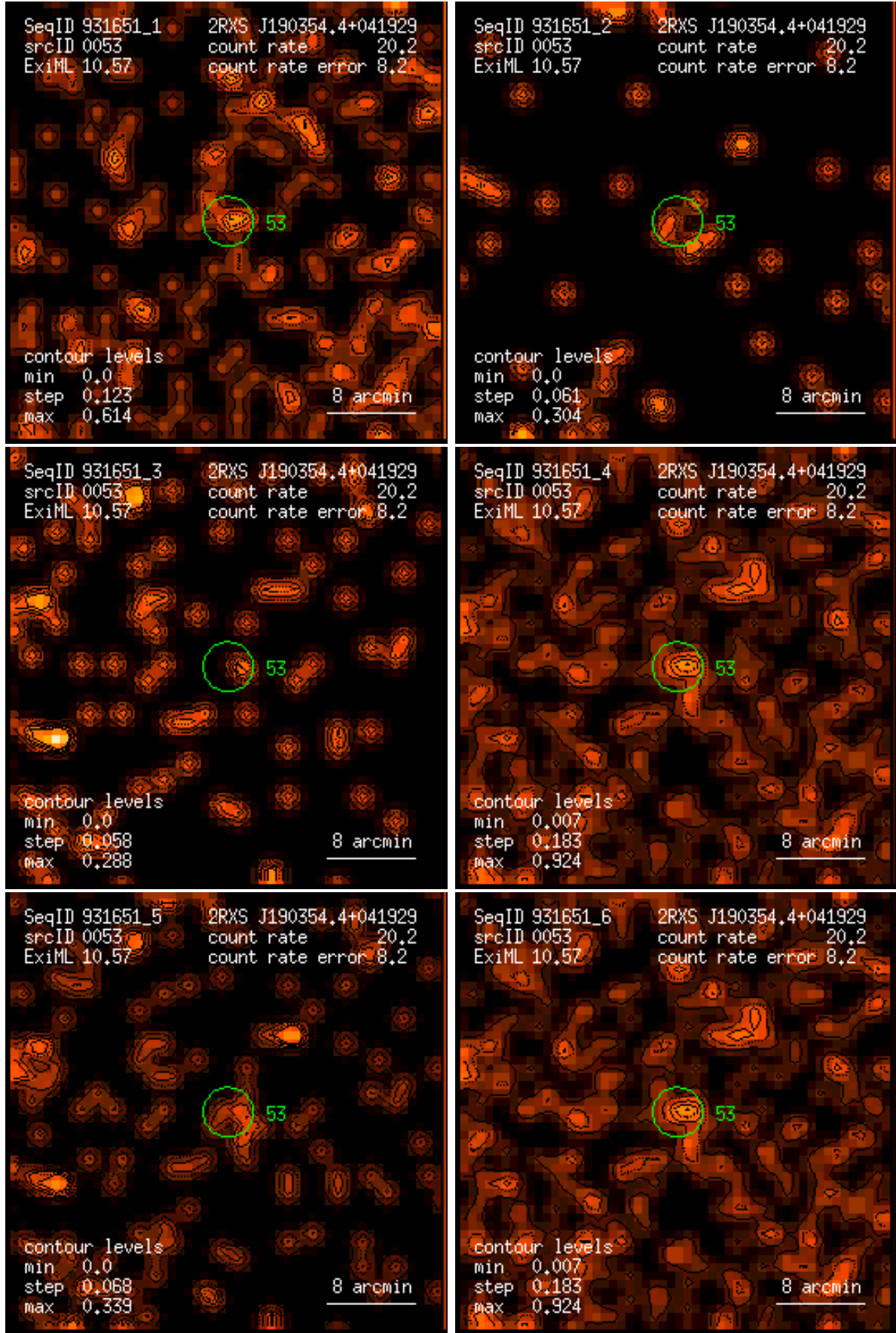
Figure 53: RASS 931651: detection 0053: band rate images, Gaussian filter: (1) PSPC channels 11 – 41, (2) 52 – 90, (3) 91 – 201, (4) 11 – 235, (5) 52 – 201, (6) 11 – 201. Broad band rates in counts/ks. Band rate contour levels in counts/ks/arcmin 2 .
