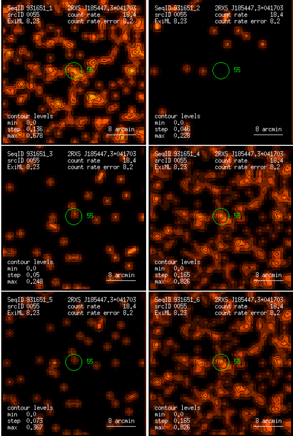
Figure 55: RASS 931651: detection 0055: band rate images, Gaussian filter: (1) PSPC channels 11 – 41, (2) 52 – 90, (3) 91 – 201, (4) 11 – 235, (5) 52 – 201, (6) 11 – 201. Broad band rates in counts/ks. Band rate contour levels in counts/ks/arcmin 2 .
