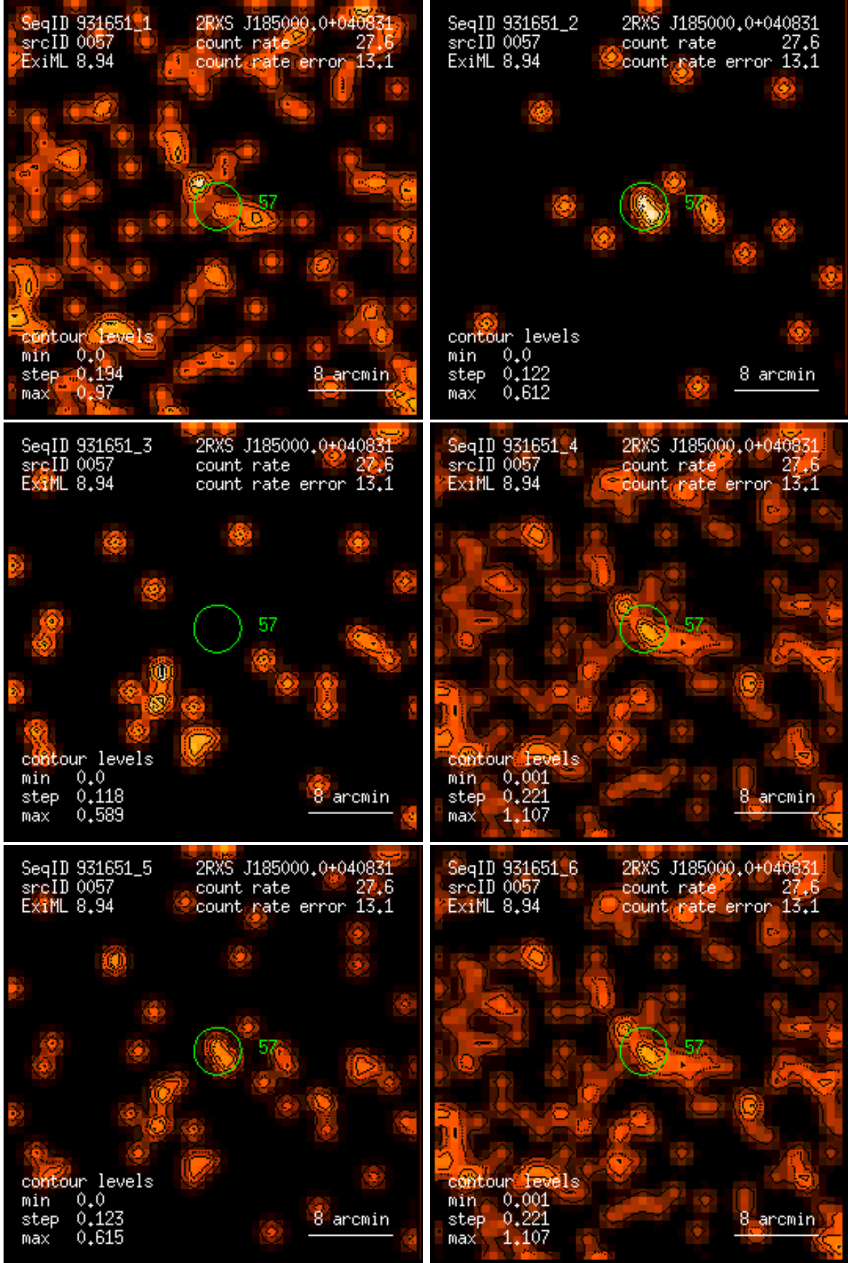
Figure 57: RASS 931651: detection 0057: band rate images, Gaussian filter: (1) PSPC channels 11 – 41, (2) 52 – 90, (3) 91 – 201, (4) 11 – 235, (5) 52 – 201, (6) 11 – 201. Broad band rates in counts/ks. Band rate contour levels in counts/ks/arcmin 2 .
