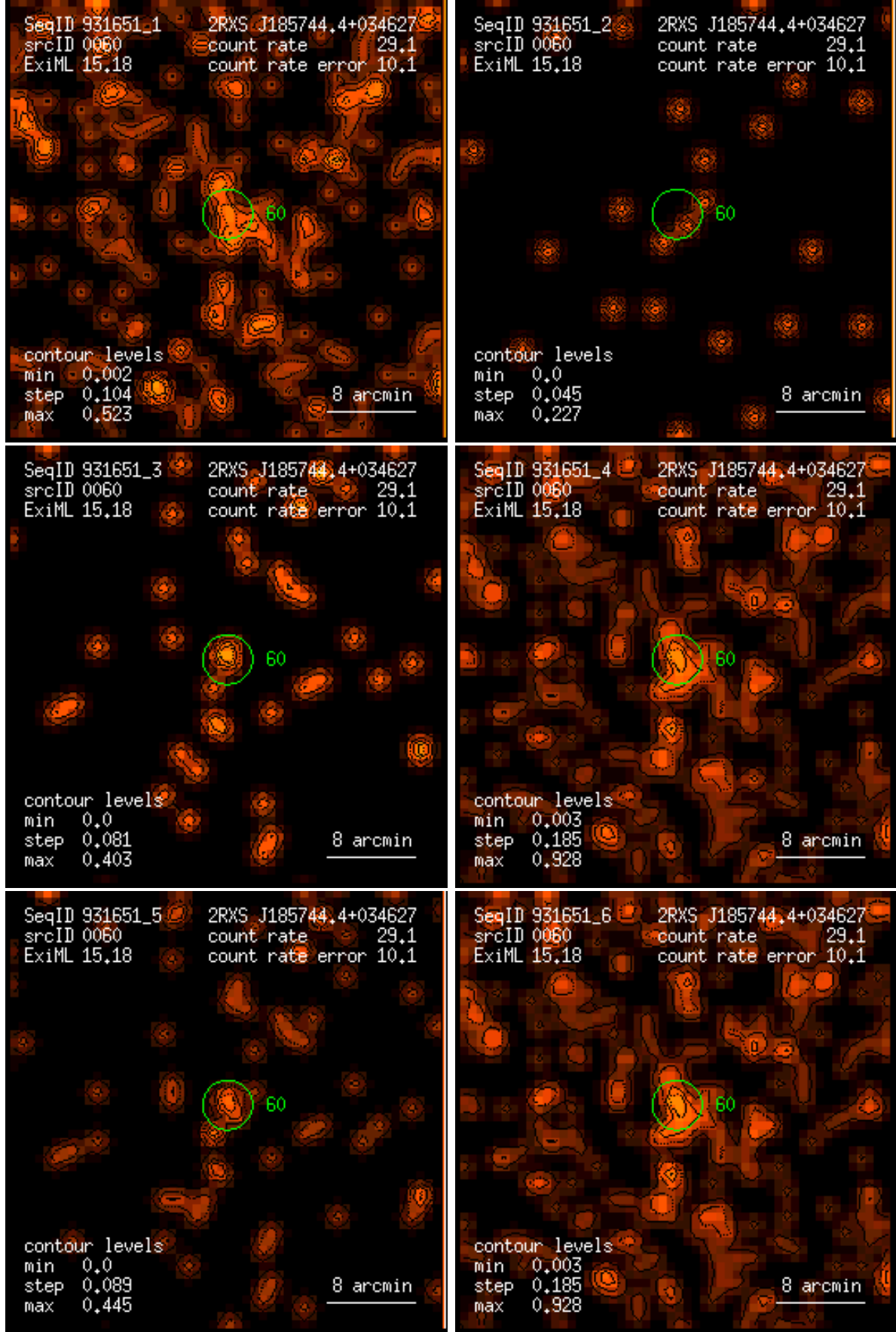
Figure 60: RASS 931651: detection 0060: band rate images, Gaussian filter: (1) PSPC channels 11 – 41, (2) 52 – 90, (3) 91 – 201, (4) 11 – 235, (5) 52 – 201, (6) 11 – 201. Broad band rates in counts/ks. Band rate contour levels in counts/ks/arcmin 2 .
