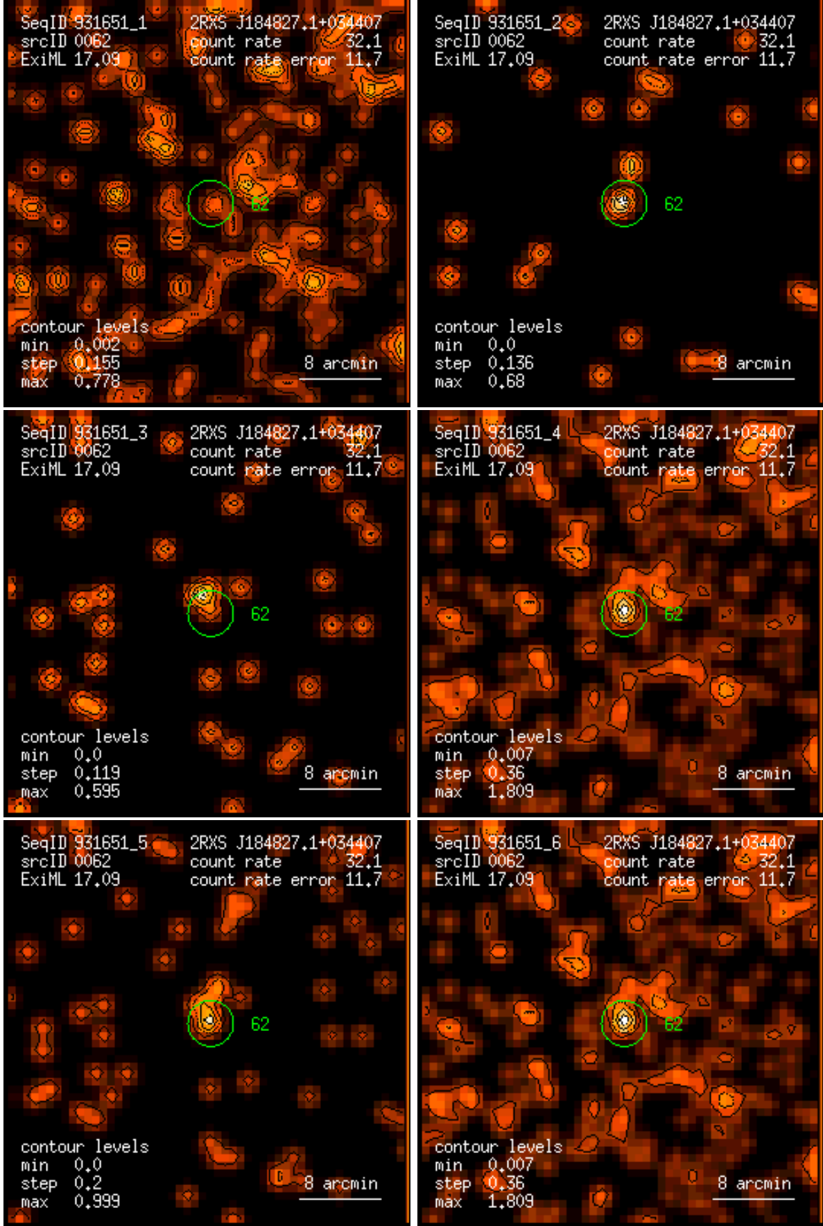
Figure 62: RASS 931651: detection 0062: band rate images, Gaussian filter: (1) PSPC channels 11 – 41, (2) 52 – 90, (3) 91 – 201, (4) 11 – 235, (5) 52 – 201, (6) 11 – 201. Broad band rates in counts/ks. Band rate contour levels in counts/ks/arcmin 2 .
