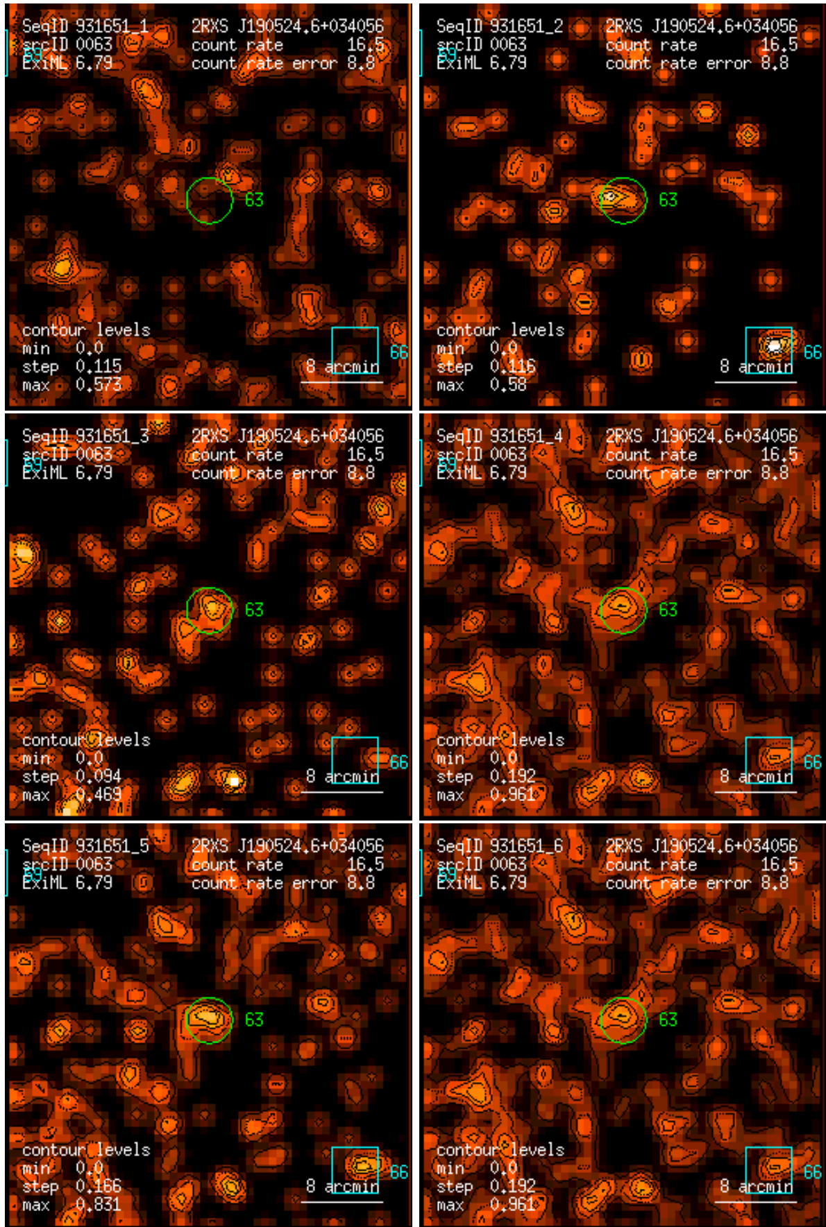
Figure 63: RASS 931651: detection 0063: band rate images, Gaussian filter: (1) PSPC channels 11 – 41, (2) 52 – 90, (3) 91 – 201, (4) 11 – 235, (5) 52 – 201, (6) 11 – 201. Broad band rates in counts/ks. Band rate contour levels in counts/ks/arcmin 2 .
