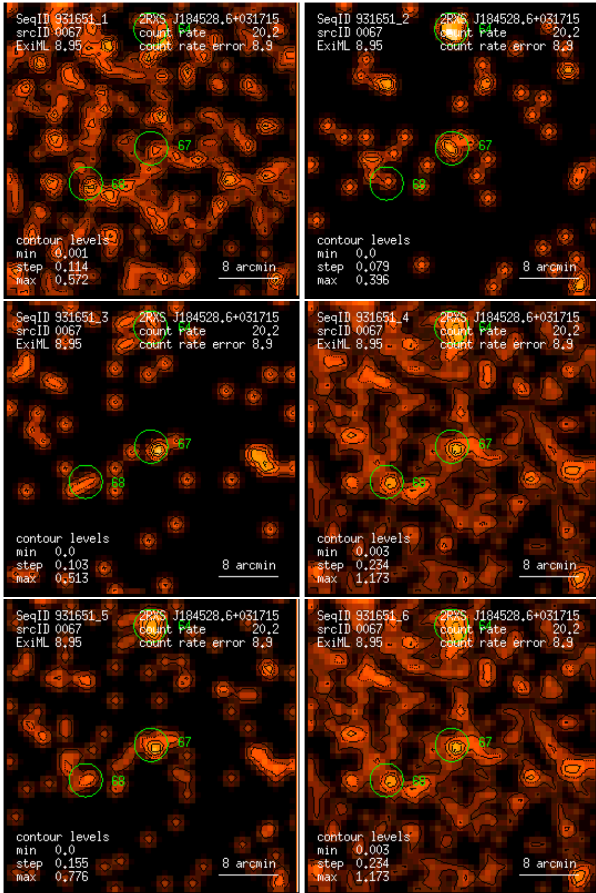
Figure 67: RASS 931651: detection 0067: band rate images, Gaussian filter: (1) PSPC channels 11 – 41, (2) 52 – 90, (3) 91 – 201, (4) 11 – 235, (5) 52 – 201, (6) 11 – 201. Broad band rates in counts/ks. Band rate contour levels in counts/ks/arcmin 2 .
