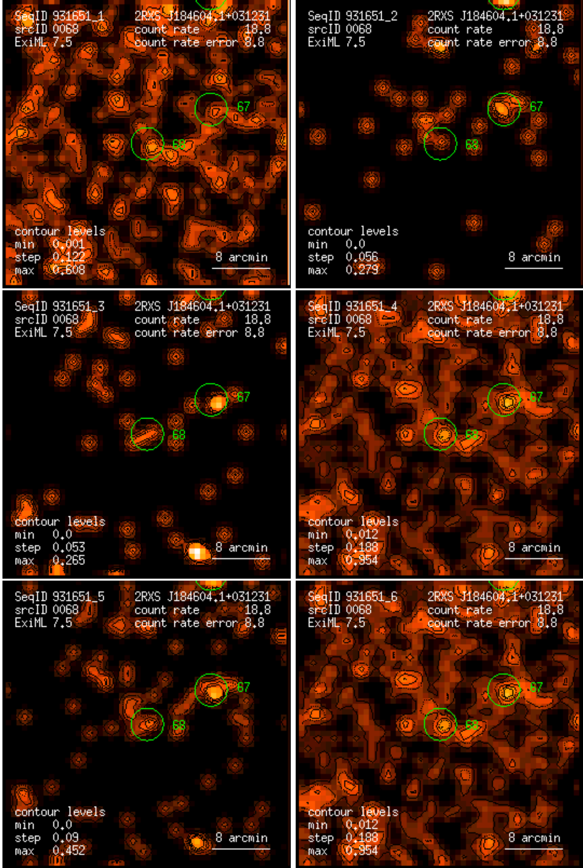
Figure 68: RASS 931651: detection 0068: band rate images, Gaussian filter: (1) PSPC channels 11 – 41, (2) 52 – 90, (3) 91 – 201, (4) 11 – 235, (5) 52 – 201, (6) 11 – 201. Broad band rates in counts/ks. Band rate contour levels in counts/ks/arcmin 2 .
