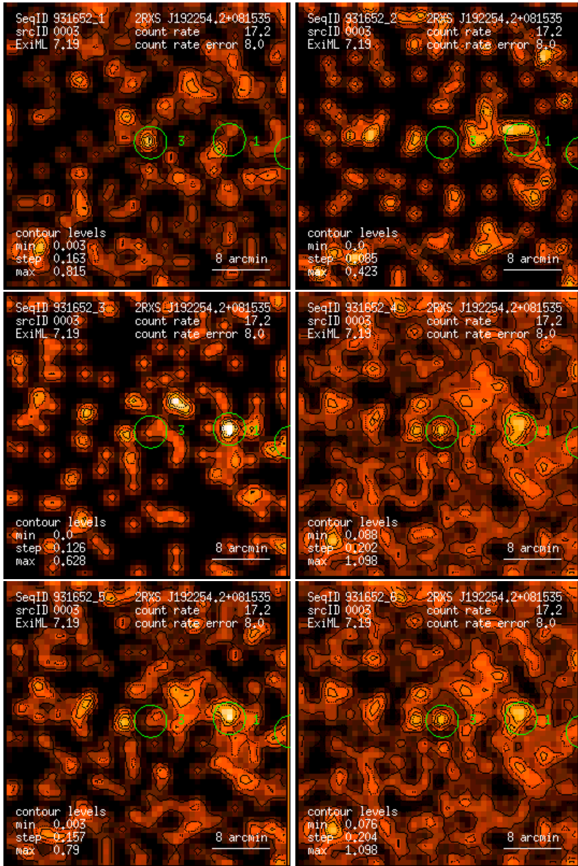
Figure 3: RASS 931652: detection 0003: band rate images, Gaussian filter: (1) PSPC channels 11 – 41, (2) 52 – 90, (3) 91 – 201, (4) 11 – 235, (5) 52 – 201, (6) 11 – 201. Broad band rates in counts/ks. Band rate contour levels in counts/ks/arcmin 2 .
