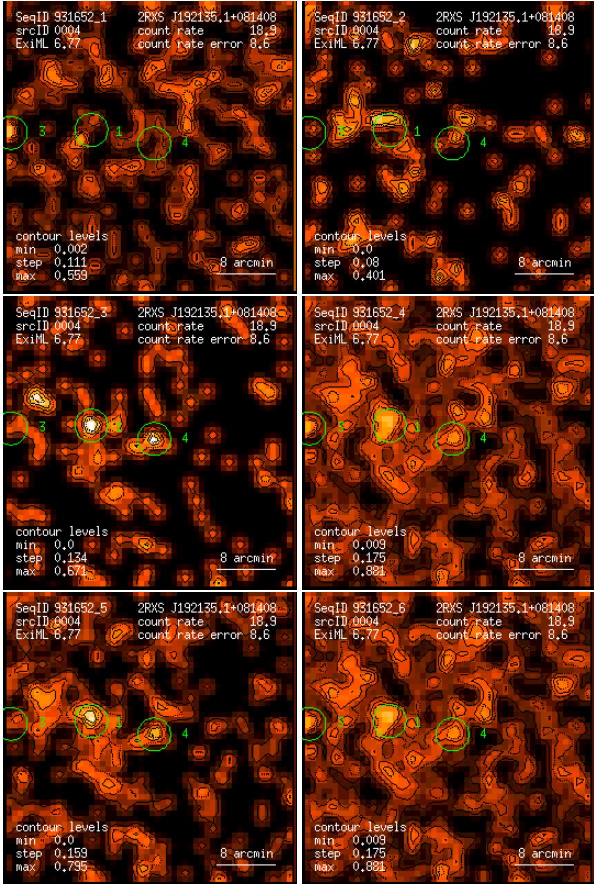
Figure 4: RASS 931652: detection 0004: band rate images, Gaussian filter: (1) PSPC channels 11 – 41, (2) 52 – 90, (3) 91 – 201, (4) 11 – 235, (5) 52 – 201, (6) 11 – 201. Broad band rates in counts/ks. Band rate contour levels in counts/ks/arcmin 2 .
