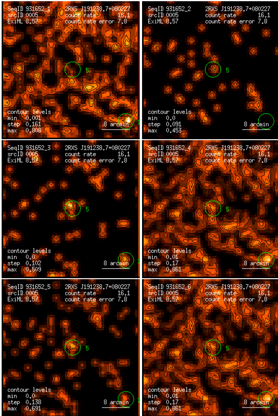
Figure 5: RASS 931652: detection 0005: band rate images, Gaussian filter: (1) PSPC channels 11 – 41, (2) 52 – 90, (3) 91 – 201, (4) 11 – 235, (5) 52 – 201, (6) 11 – 201. Broad band rates in counts/ks. Band rate contour levels in counts/ks/arcmin 2 .
