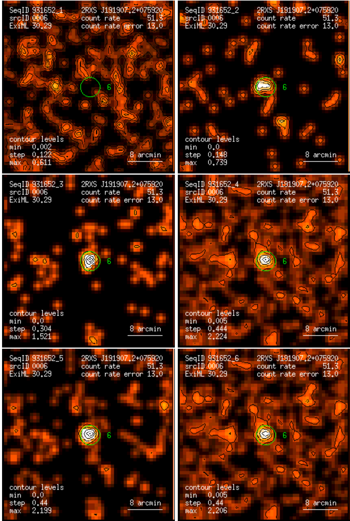
Figure 6: RASS 931652: detection 0006: band rate images, Gaussian filter: (1) PSPC channels 11 – 41, (2) 52 – 90, (3) 91 – 201, (4) 11 – 235, (5) 52 – 201, (6) 11 – 201. Broad band rates in counts/ks. Band rate contour levels in counts/ks/arcmin 2 .
