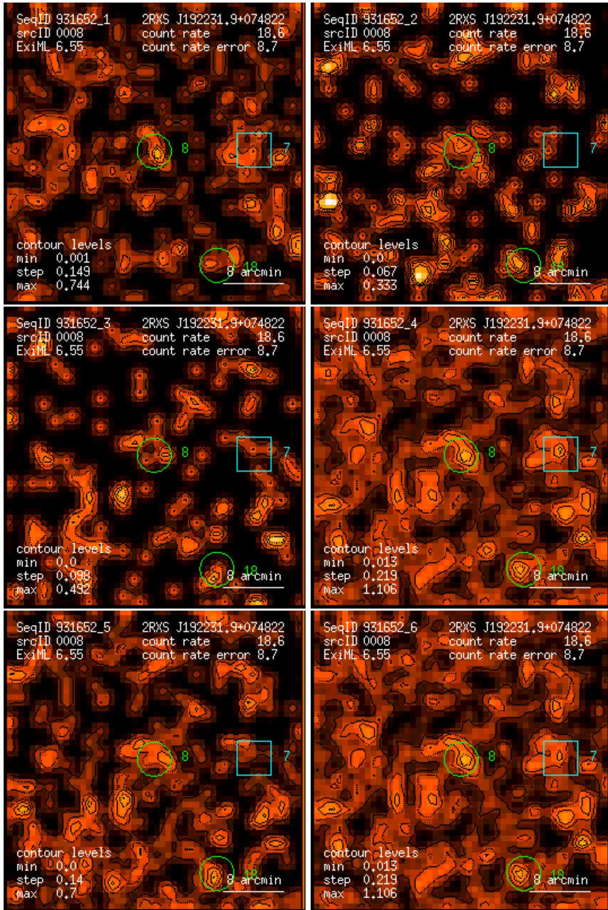
Figure 8: RASS 931652: detection 0008: band rate images, Gaussian filter: (1) PSPC channels 11 – 41, (2) 52 – 90, (3) 91 – 201, (4) 11 – 235, (5) 52 – 201, (6) 11 – 201. Broad band rates in counts/ks. Band rate contour levels in counts/ks/arcmin 2 .
