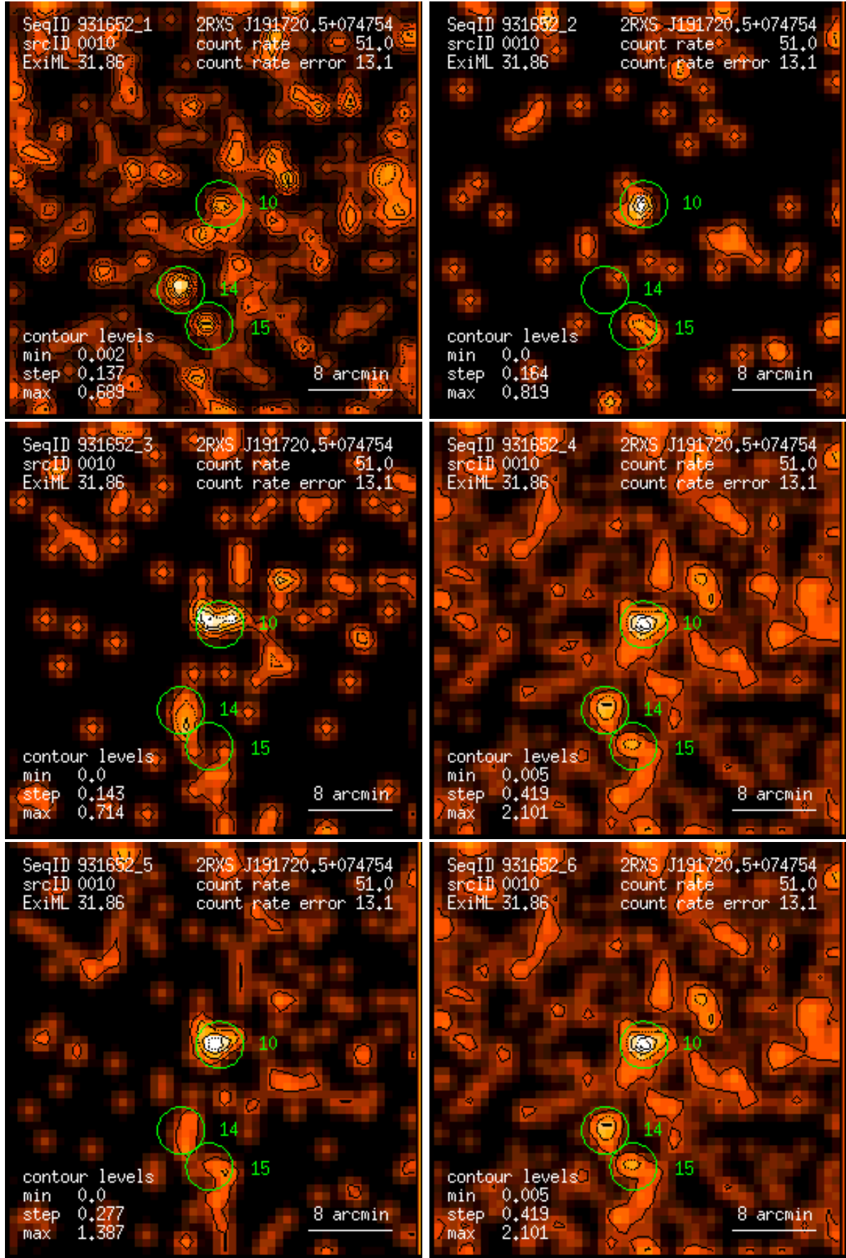
Figure 10: RASS 931652: detection 0010: band rate images, Gaussian filter: (1) PSPC channels 11 – 41, (2) 52 – 90, (3) 91 – 201, (4) 11 – 235, (5) 52 – 201, (6) 11 – 201. Broad band rates in counts/ks. Band rate contour levels in counts/ks/arcmin 2 .
