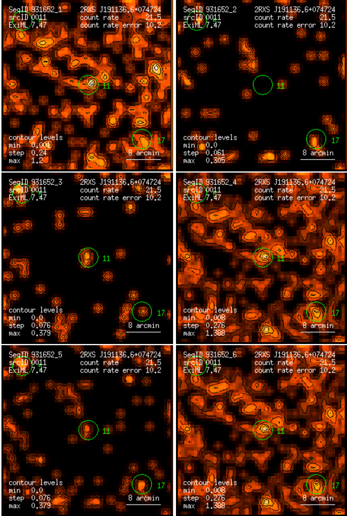
Figure 11: RASS 931652: detection 0011: band rate images, Gaussian filter: (1) PSPC channels 11 – 41, (2) 52 – 90, (3) 91 – 201, (4) 11 – 235, (5) 52 – 201, (6) 11 – 201. Broad band rates in counts/ks. Band rate contour levels in counts/ks/arcmin 2 .
