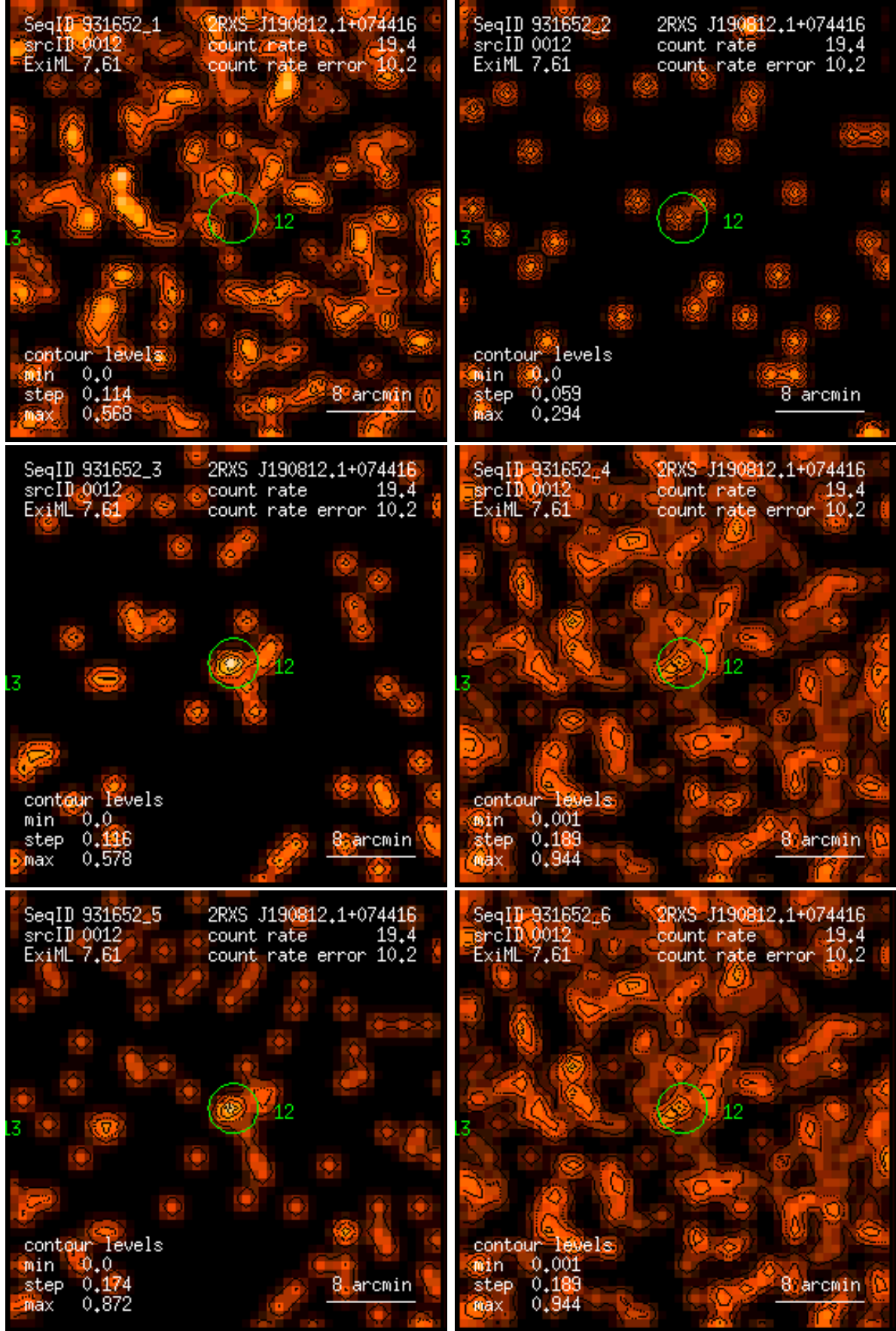
Figure 12: RASS 931652: detection 0012: band rate images, Gaussian filter: (1) PSPC channels 11 – 41, (2) 52 – 90, (3) 91 – 201, (4) 11 – 235, (5) 52 – 201, (6) 11 – 201. Broad band rates in counts/ks. Band rate contour levels in counts/ks/arcmin 2 .
