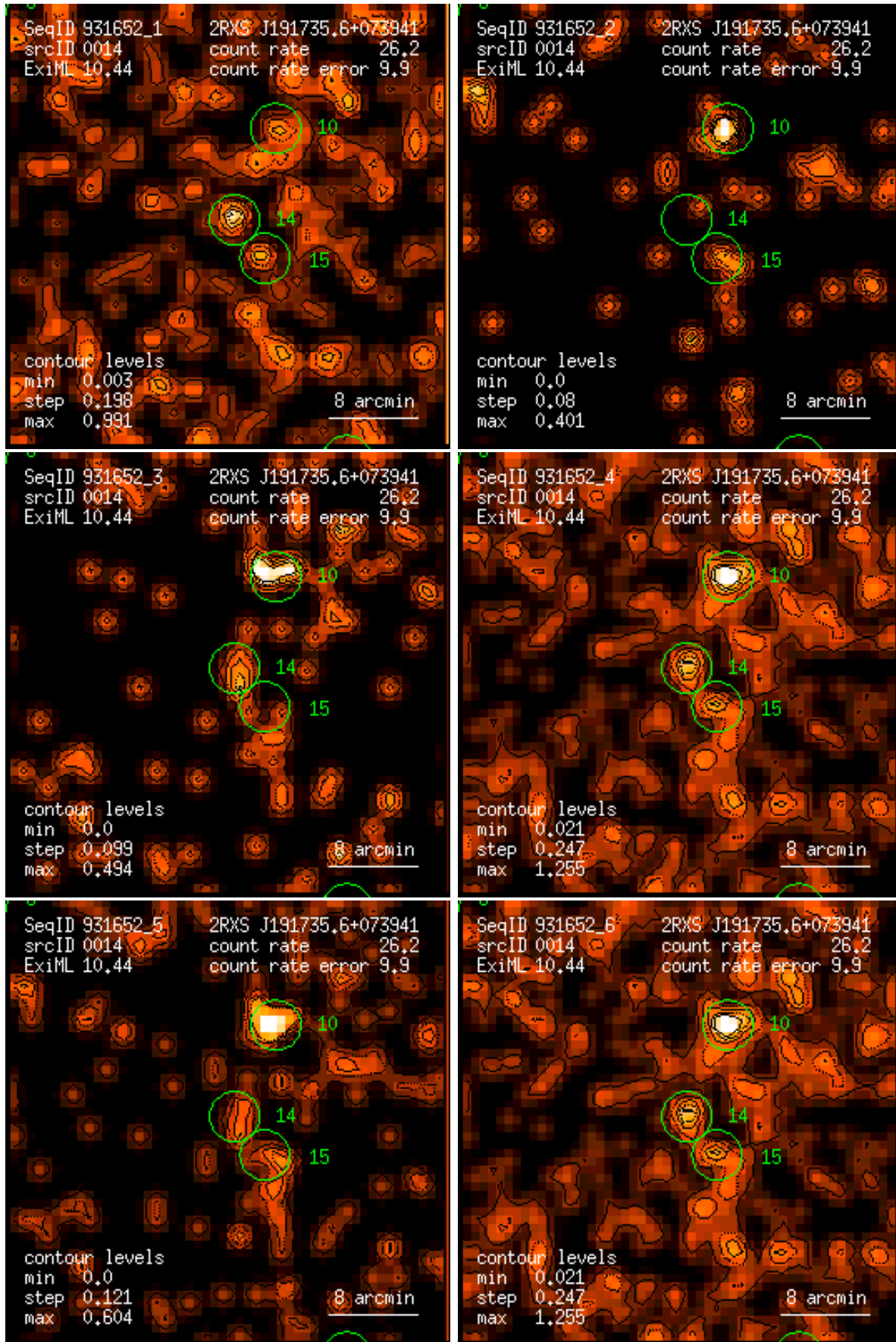
Figure 14: RASS 931652: detection 0014: band rate images, Gaussian filter: (1) PSPC channels 11 – 41, (2) 52 – 90, (3) 91 – 201, (4) 11 – 235, (5) 52 – 201, (6) 11 – 201. Broad band rates in counts/ks. Band rate contour levels in counts/ks/arcmin 2 .
