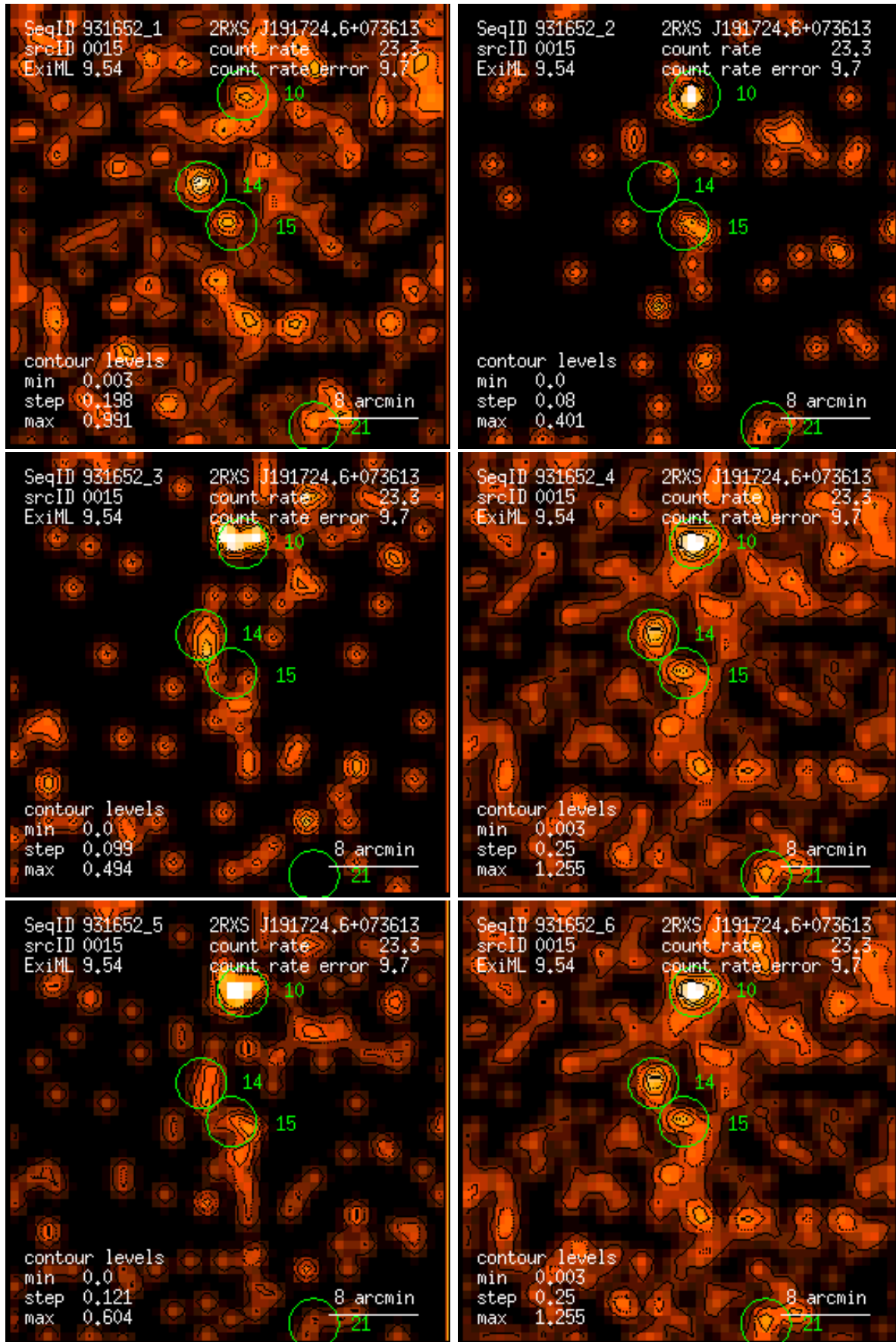
Figure 15: RASS 931652: detection 0015: band rate images, Gaussian filter: (1) PSPC channels 11 – 41, (2) 52 – 90, (3) 91 – 201, (4) 11 – 235, (5) 52 – 201, (6) 11 – 201. Broad band rates in counts/ks. Band rate contour levels in counts/ks/arcmin 2 .
