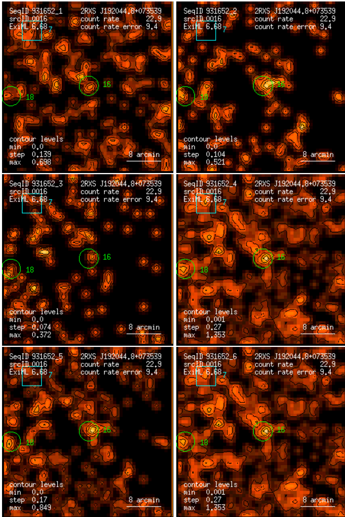
Figure 16: RASS 931652: detection 0016: band rate images, Gaussian filter: (1) PSPC channels 11 – 41, (2) 52 – 90, (3) 91 – 201, (4) 11 – 235, (5) 52 – 201, (6) 11 – 201. Broad band rates in counts/ks. Band rate contour levels in counts/ks/arcmin 2 .
