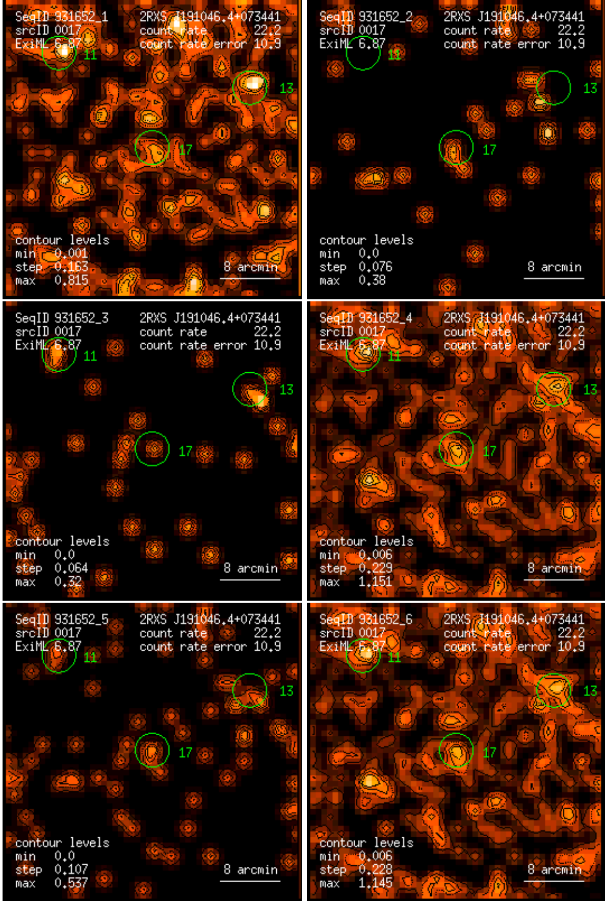
Figure 17: RASS 931652: detection 0017: band rate images, Gaussian filter: (1) PSPC channels 11 – 41, (2) 52 – 90, (3) 91 – 201, (4) 11 – 235, (5) 52 – 201, (6) 11 – 201. Broad band rates in counts/ks. Band rate contour levels in counts/ks/arcmin 2 .
