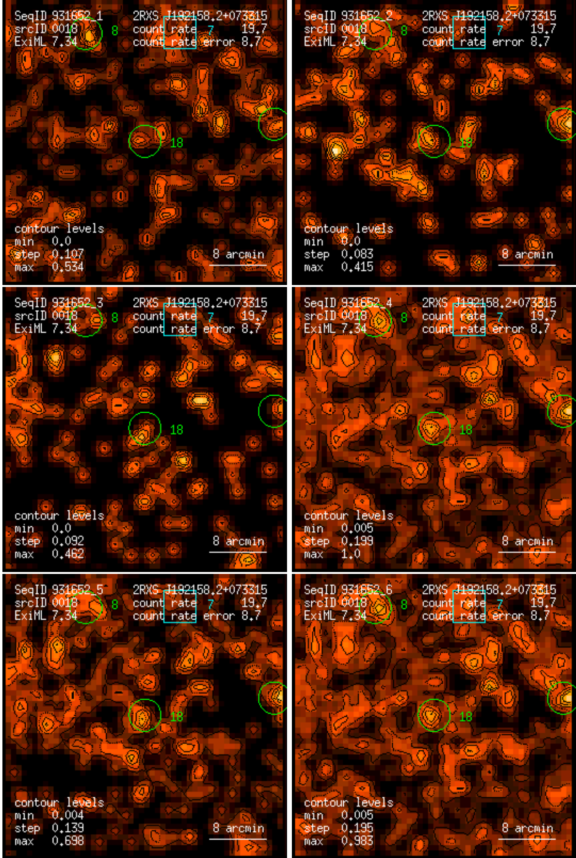
Figure 18: RASS 931652: detection 0018: band rate images, Gaussian filter: (1) PSPC channels 11 – 41, (2) 52 – 90, (3) 91 – 201, (4) 11 – 235, (5) 52 – 201, (6) 11 – 201. Broad band rates in counts/ks. Band rate contour levels in counts/ks/arcmin 2 .
