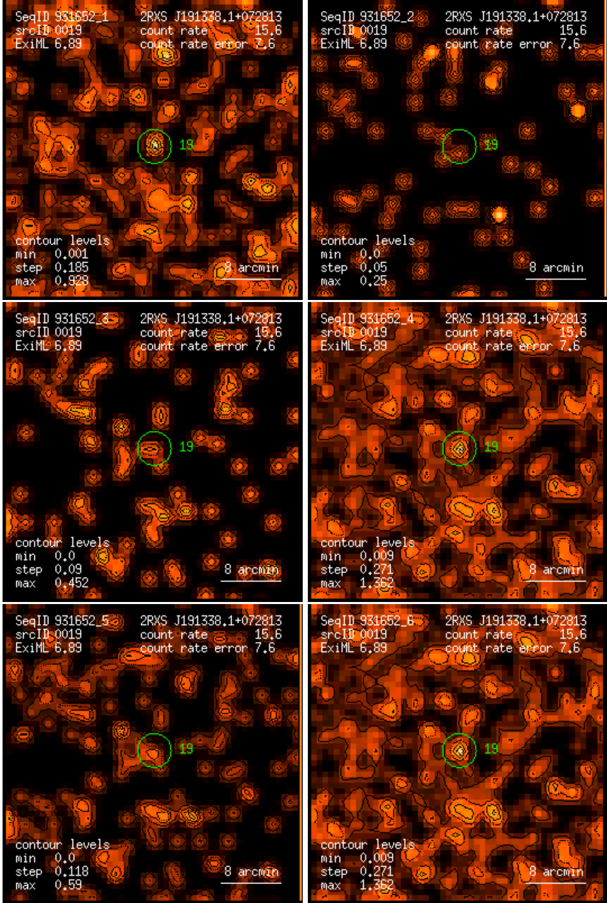
Figure 19: RASS 931652: detection 0019: band rate images, Gaussian filter: (1) PSPC channels 11 – 41, (2) 52 – 90, (3) 91 – 201, (4) 11 – 235, (5) 52 – 201, (6) 11 – 201. Broad band rates in counts/ks. Band rate contour levels in counts/ks/arcmin 2 .
