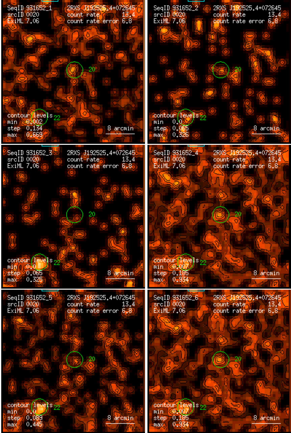
Figure 20: RASS 931652: detection 0020: band rate images, Gaussian filter: (1) PSPC channels 11 – 41, (2) 52 – 90, (3) 91 – 201, (4) 11 – 235, (5) 52 – 201, (6) 11 – 201. Broad band rates in counts/ks. Band rate contour levels in counts/ks/arcmin 2 .
