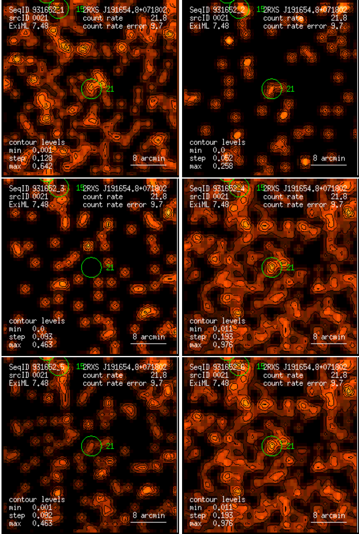
Figure 21: RASS 931652: detection 0021: band rate images, Gaussian filter: (1) PSPC channels 11 – 41, (2) 52 – 90, (3) 91 – 201, (4) 11 – 235, (5) 52 – 201, (6) 11 – 201. Broad band rates in counts/ks. Band rate contour levels in counts/ks/arcmin 2 .
