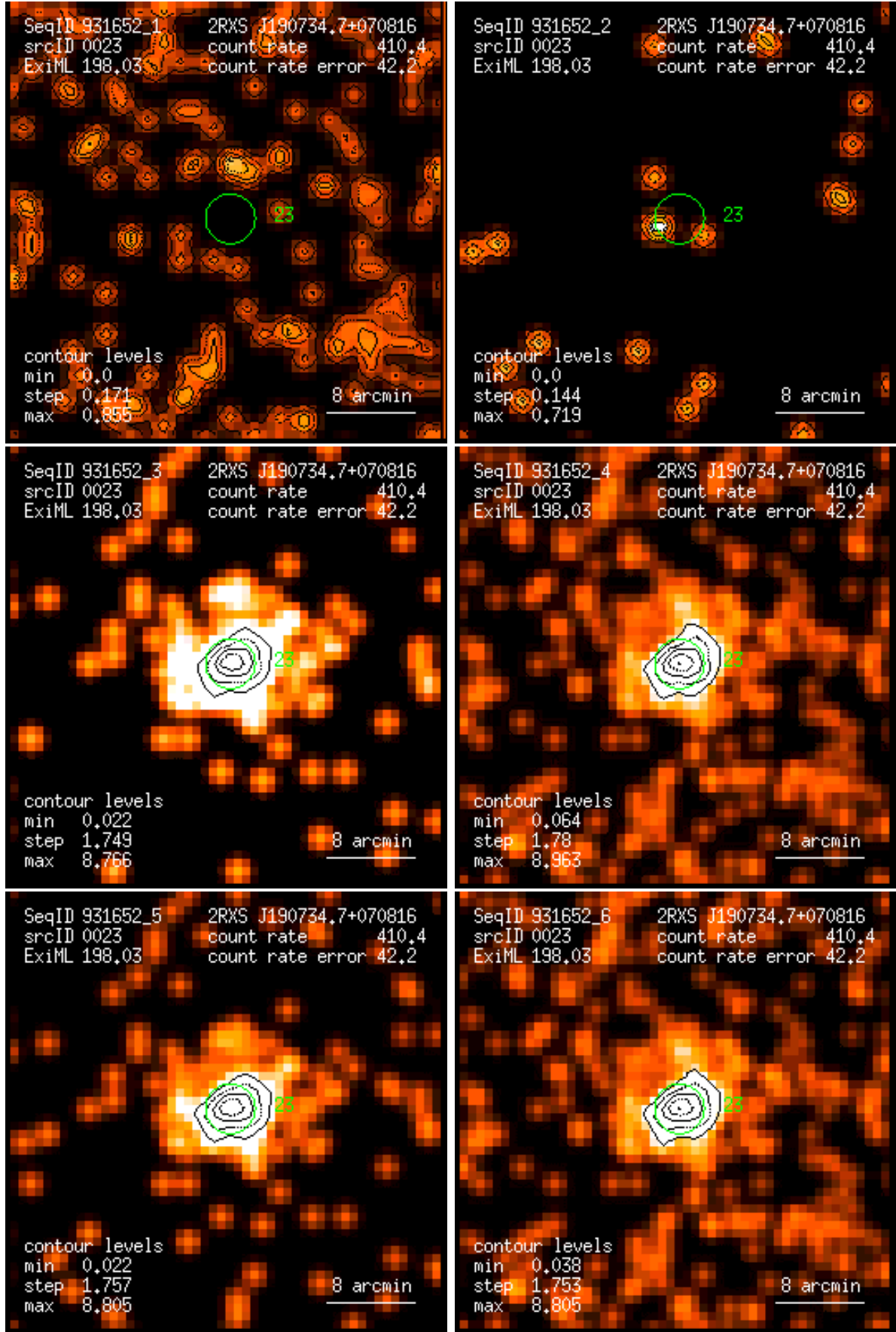
Figure 23: RASS 931652: detection 0023: band rate images, Gaussian filter: (1) PSPC channels 11 – 41, (2) 52 – 90, (3) 91 – 201, (4) 11 – 235, (5) 52 – 201, (6) 11 – 201. Broad band rates in counts/ks. Band rate contour levels in counts/ks/arcmin 2 .
