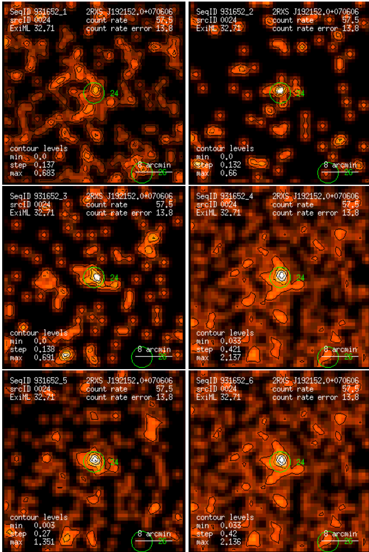
Figure 24: RASS 931652: detection 0024: band rate images, Gaussian filter: (1) PSPC channels 11 – 41, (2) 52 – 90, (3) 91 – 201, (4) 11 – 235, (5) 52 – 201, (6) 11 – 201. Broad band rates in counts/ks. Band rate contour levels in counts/ks/arcmin 2 .
