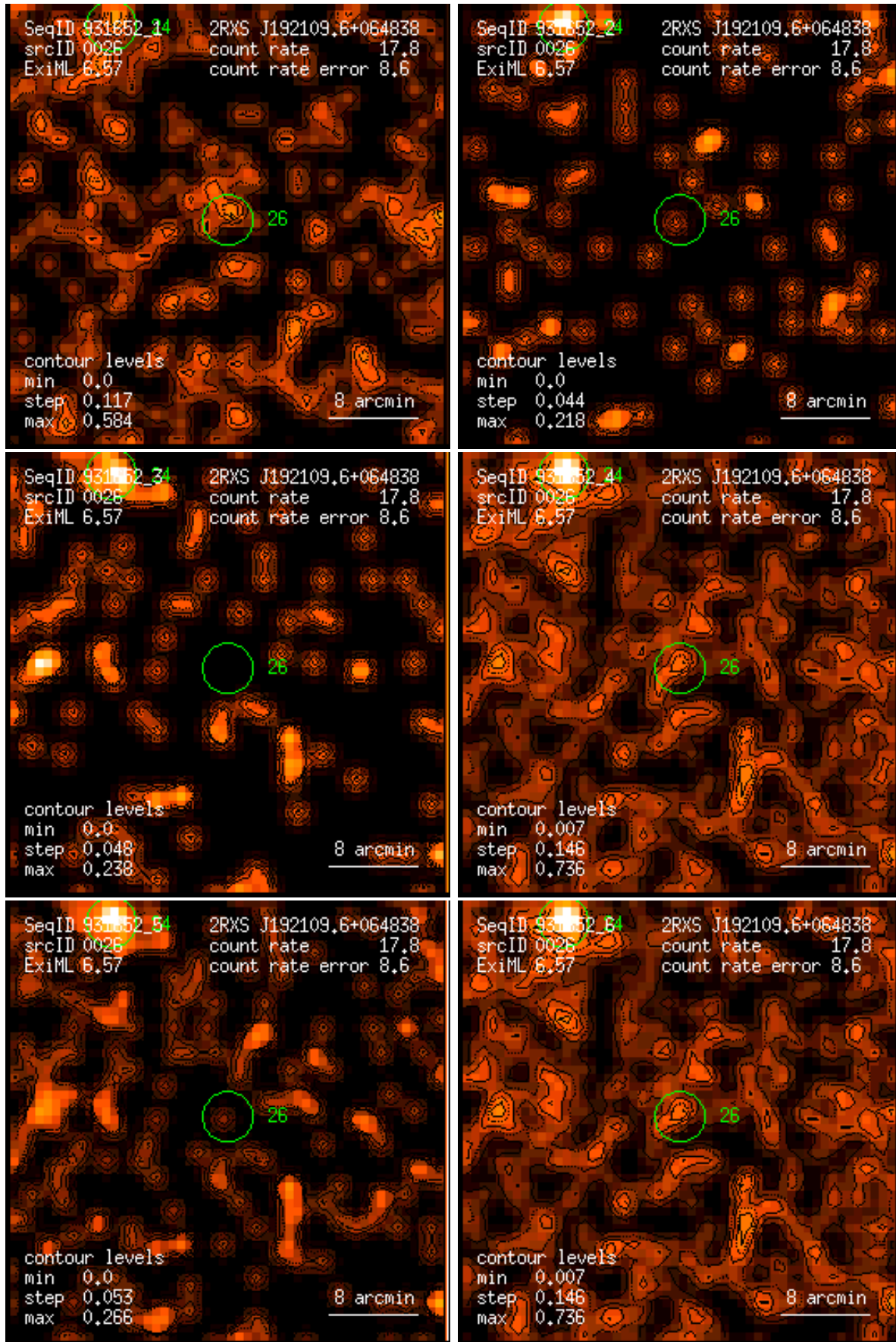
Figure 26: RASS 931652: detection 0026: band rate images, Gaussian filter: (1) PSPC channels 11 – 41, (2) 52 – 90, (3) 91 – 201, (4) 11 – 235, (5) 52 – 201, (6) 11 – 201. Broad band rates in counts/ks. Band rate contour levels in counts/ks/arcmin 2 .
