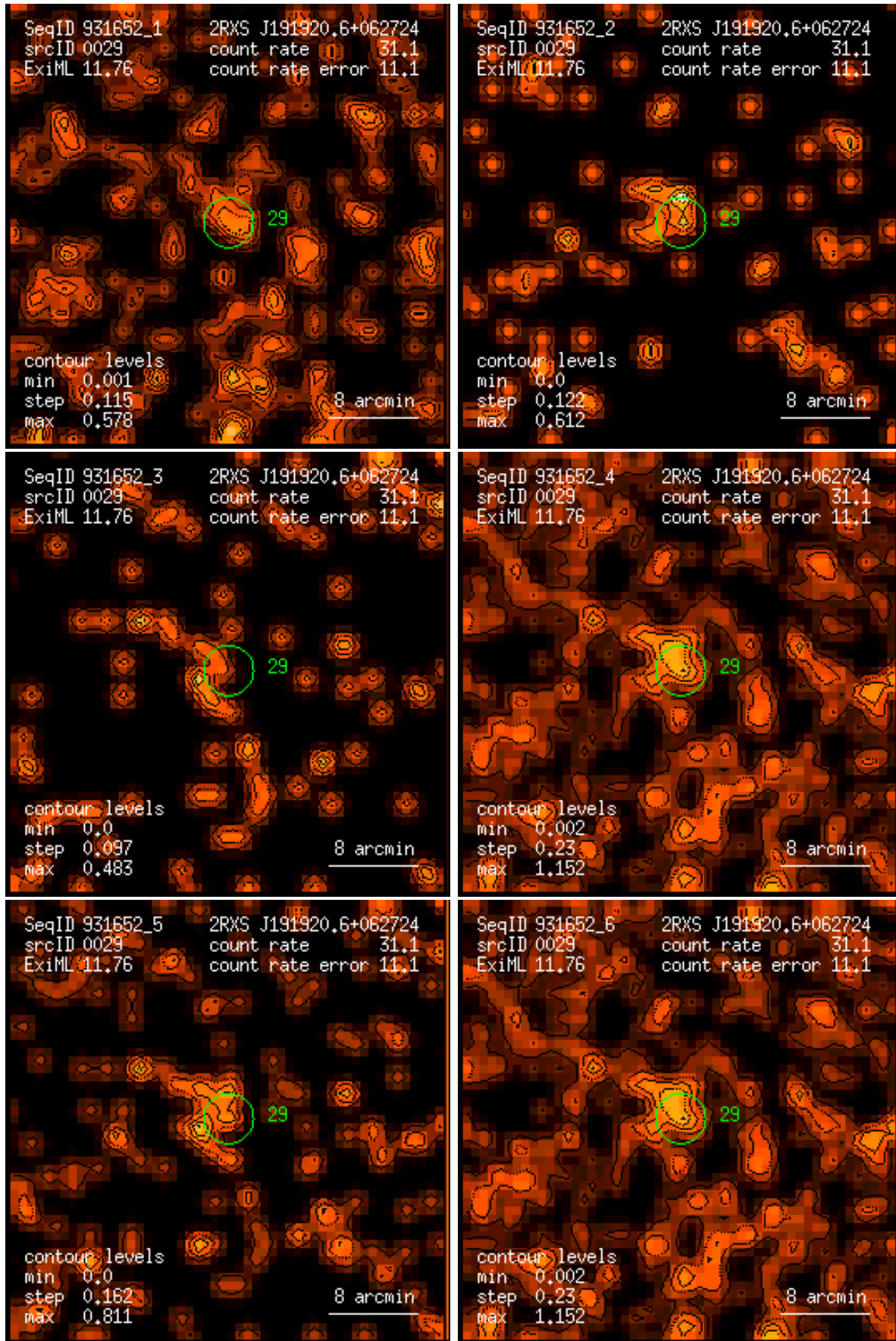
Figure 29: RASS 931652: detection 0029: band rate images, Gaussian filter: (1) PSPC channels 11 – 41, (2) 52 – 90, (3) 91 – 201, (4) 11 – 235, (5) 52 – 201, (6) 11 – 201. Broad band rates in counts/ks. Band rate contour levels in counts/ks/arcmin 2 .
