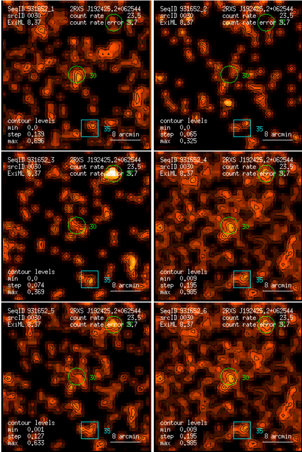
Figure 30: RASS 931652: detection 0030: band rate images, Gaussian filter: (1) PSPC channels 11 – 41, (2) 52 – 90, (3) 91 – 201, (4) 11 – 235, (5) 52 – 201, (6) 11 – 201. Broad band rates in counts/ks. Band rate contour levels in counts/ks/arcmin 2 .
