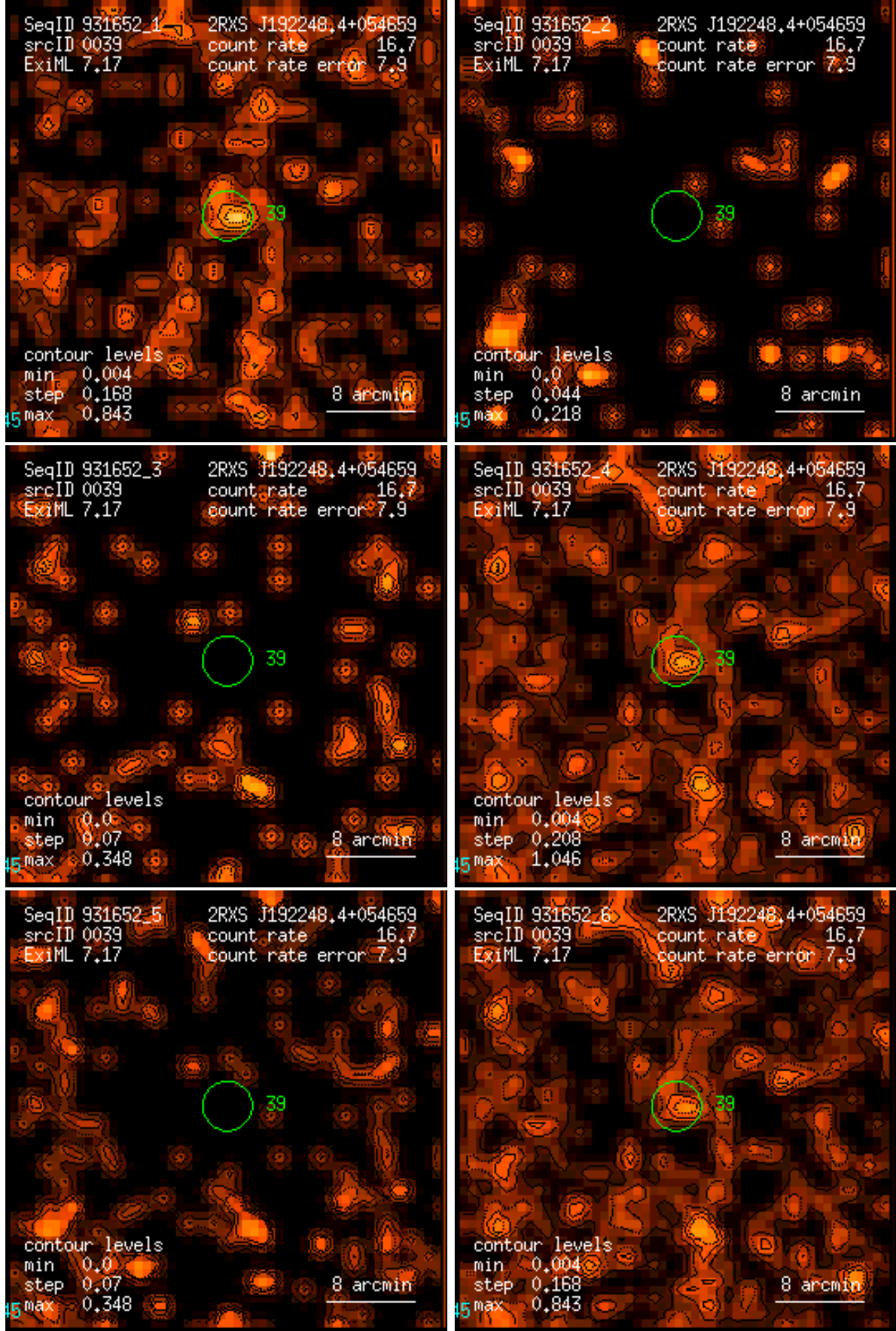
Figure 39: RASS 931652: detection 0039: band rate images, Gaussian filter: (1) PSPC channels 11 – 41, (2) 52 – 90, (3) 91 – 201, (4) 11 – 235, (5) 52 – 201, (6) 11 – 201. Broad band rates in counts/ks. Band rate contour levels in counts/ks/arcmin 2 .
