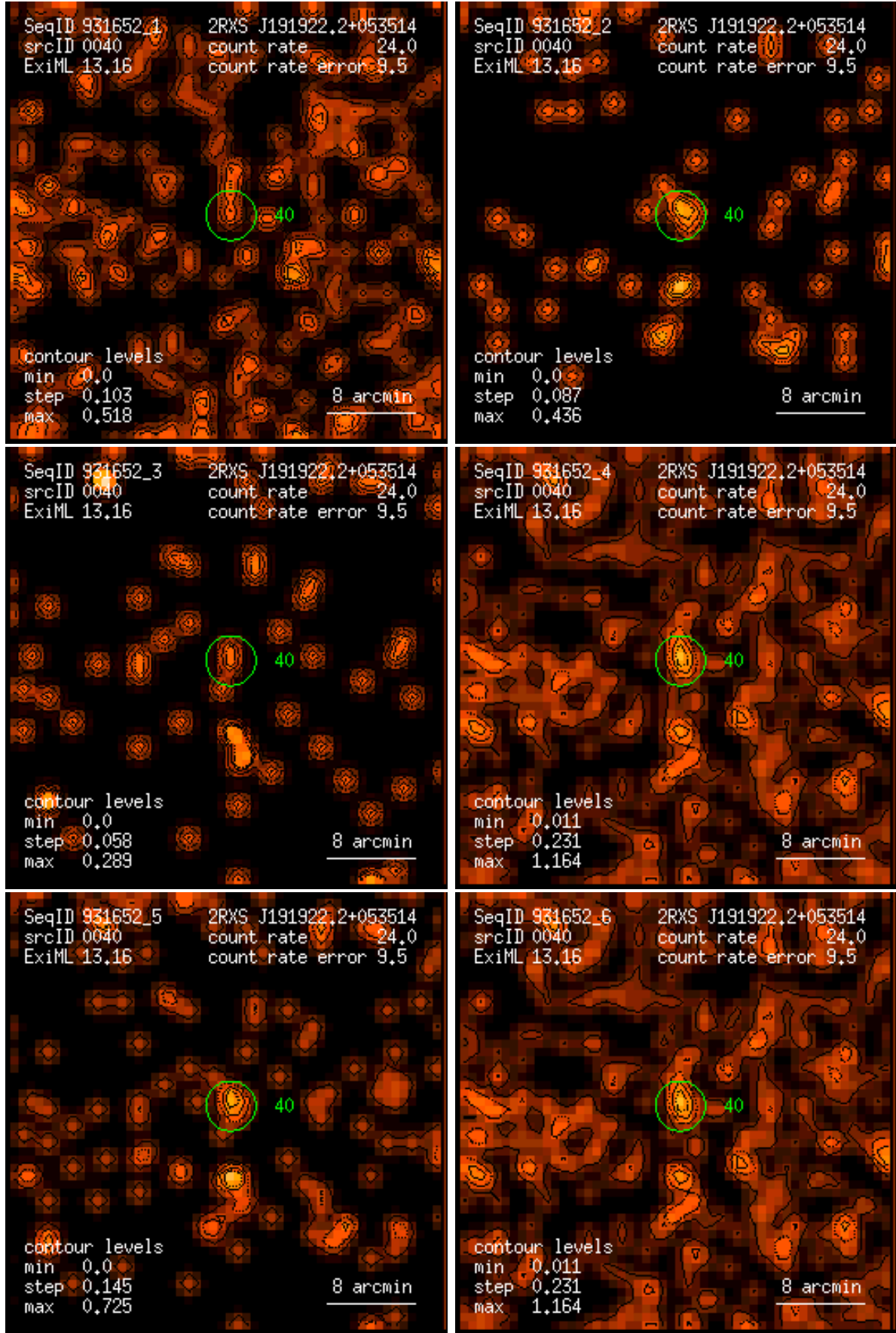
Figure 40: RASS 931652: detection 0040: band rate images, Gaussian filter: (1) PSPC channels 11 – 41, (2) 52 – 90, (3) 91 – 201, (4) 11 – 235, (5) 52 – 201, (6) 11 – 201. Broad band rates in counts/ks. Band rate contour levels in counts/ks/arcmin 2 .
