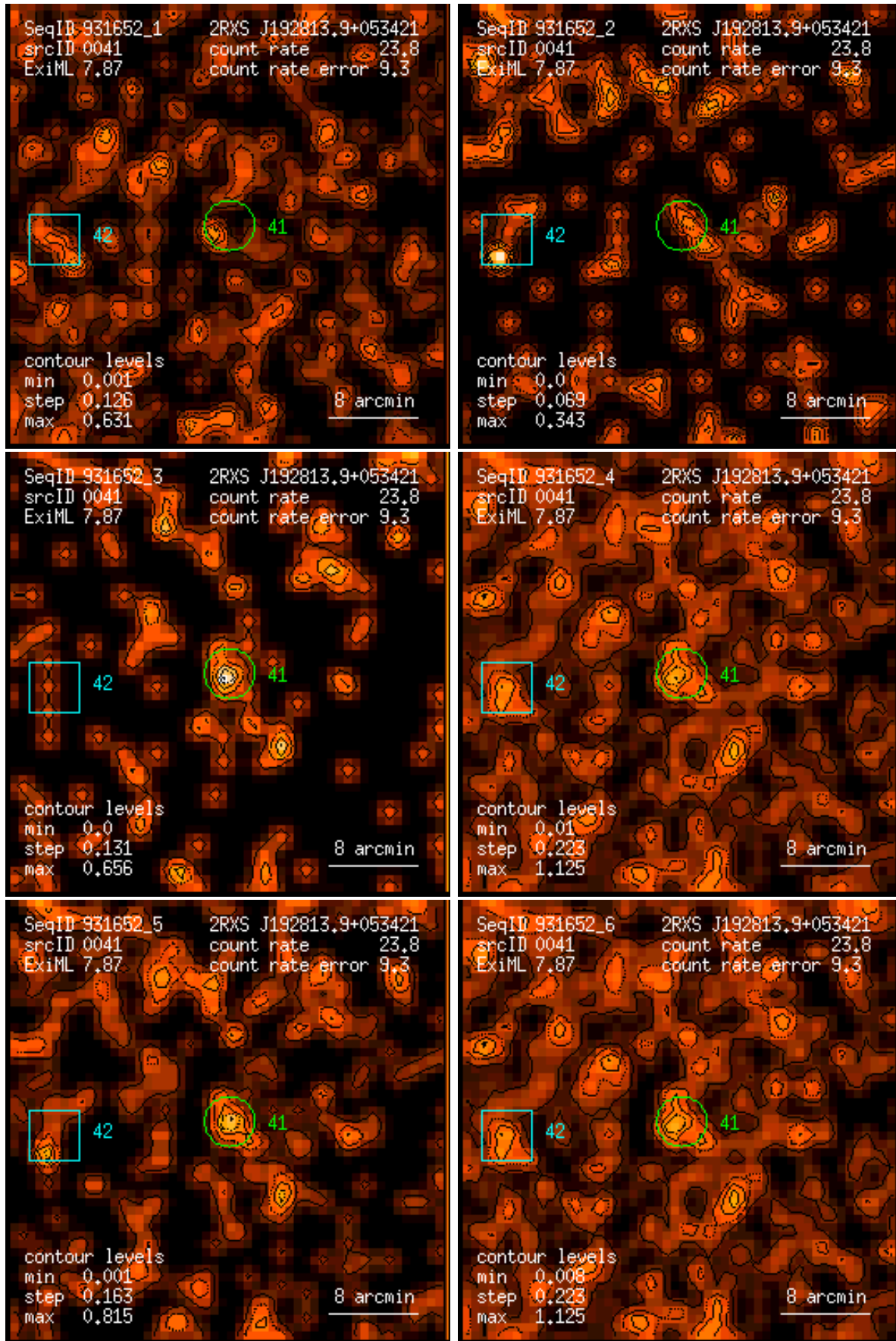
Figure 41: RASS 931652: detection 0041: band rate images, Gaussian filter: (1) PSPC channels 11 – 41, (2) 52 – 90, (3) 91 – 201, (4) 11 – 235, (5) 52 – 201, (6) 11 – 201. Broad band rates in counts/ks. Band rate contour levels in counts/ks/arcmin 2 .
