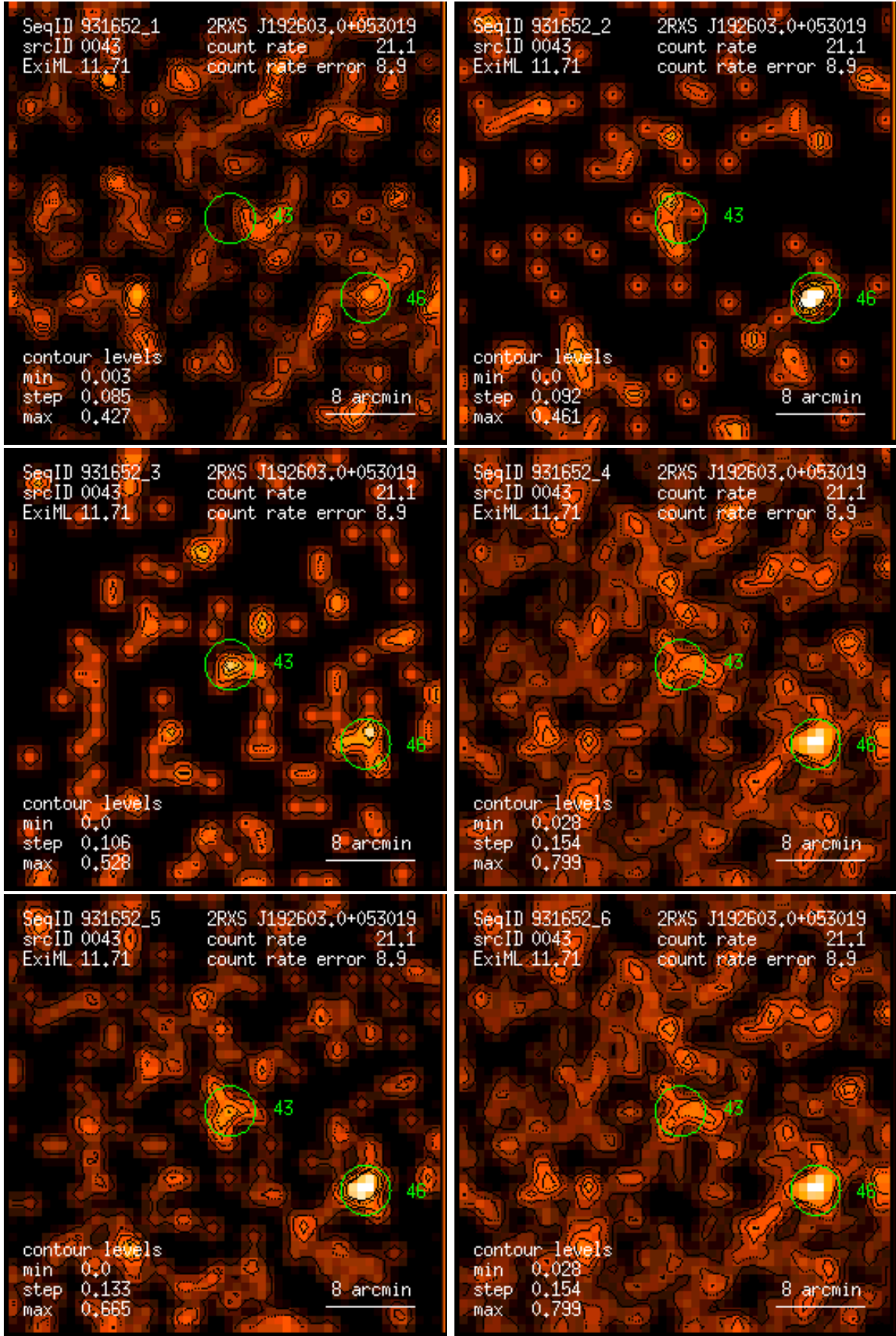
Figure 43: RASS 931652: detection 0043: band rate images, Gaussian filter: (1) PSPC channels 11 – 41, (2) 52 – 90, (3) 91 – 201, (4) 11 – 235, (5) 52 – 201, (6) 11 – 201. Broad band rates in counts/ks. Band rate contour levels in counts/ks/arcmin 2 .
