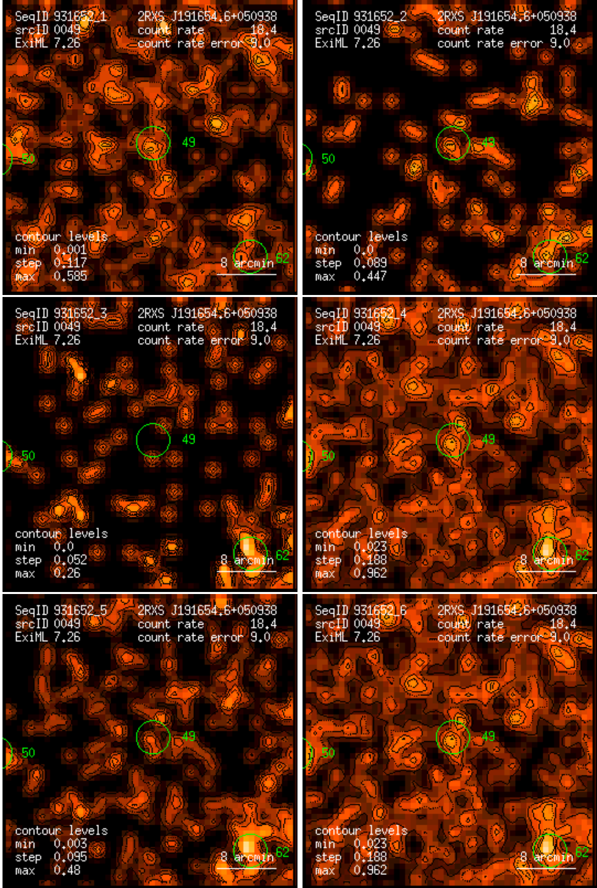
Figure 49: RASS 931652: detection 0049: band rate images, Gaussian filter: (1) PSPC channels 11 – 41, (2) 52 – 90, (3) 91 – 201, (4) 11 – 235, (5) 52 – 201, (6) 11 – 201. Broad band rates in counts/ks. Band rate contour levels in counts/ks/arcmin 2 .
