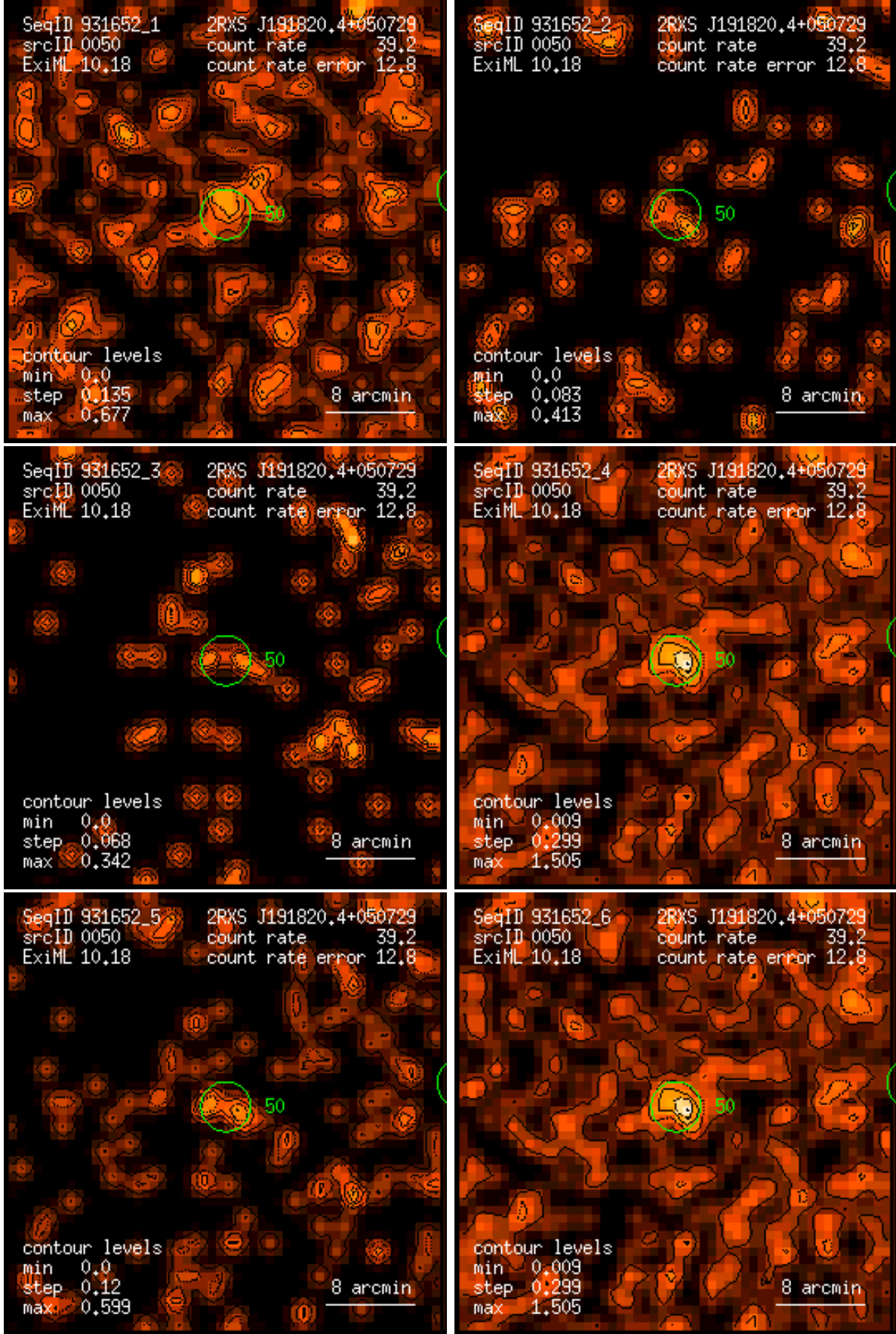
Figure 50: RASS 931652: detection 0050: band rate images, Gaussian filter: (1) PSPC channels 11 – 41, (2) 52 – 90, (3) 91 – 201, (4) 11 – 235, (5) 52 – 201, (6) 11 – 201. Broad band rates in counts/ks. Band rate contour levels in counts/ks/arcmin 2 .
