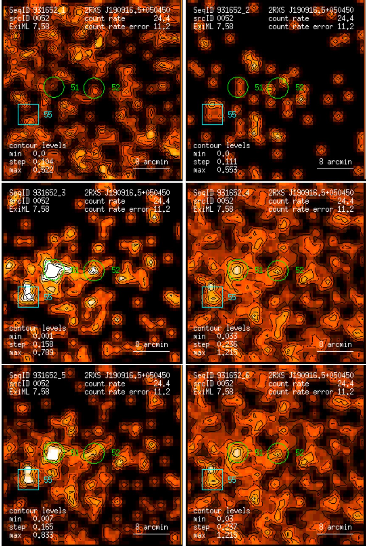
Figure 52: RASS 931652: detection 0052: band rate images, Gaussian filter: (1) PSPC channels 11 – 41, (2) 52 – 90, (3) 91 – 201, (4) 11 – 235, (5) 52 – 201, (6) 11 – 201. Broad band rates in counts/ks. Band rate contour levels in counts/ks/arcmin 2 .
