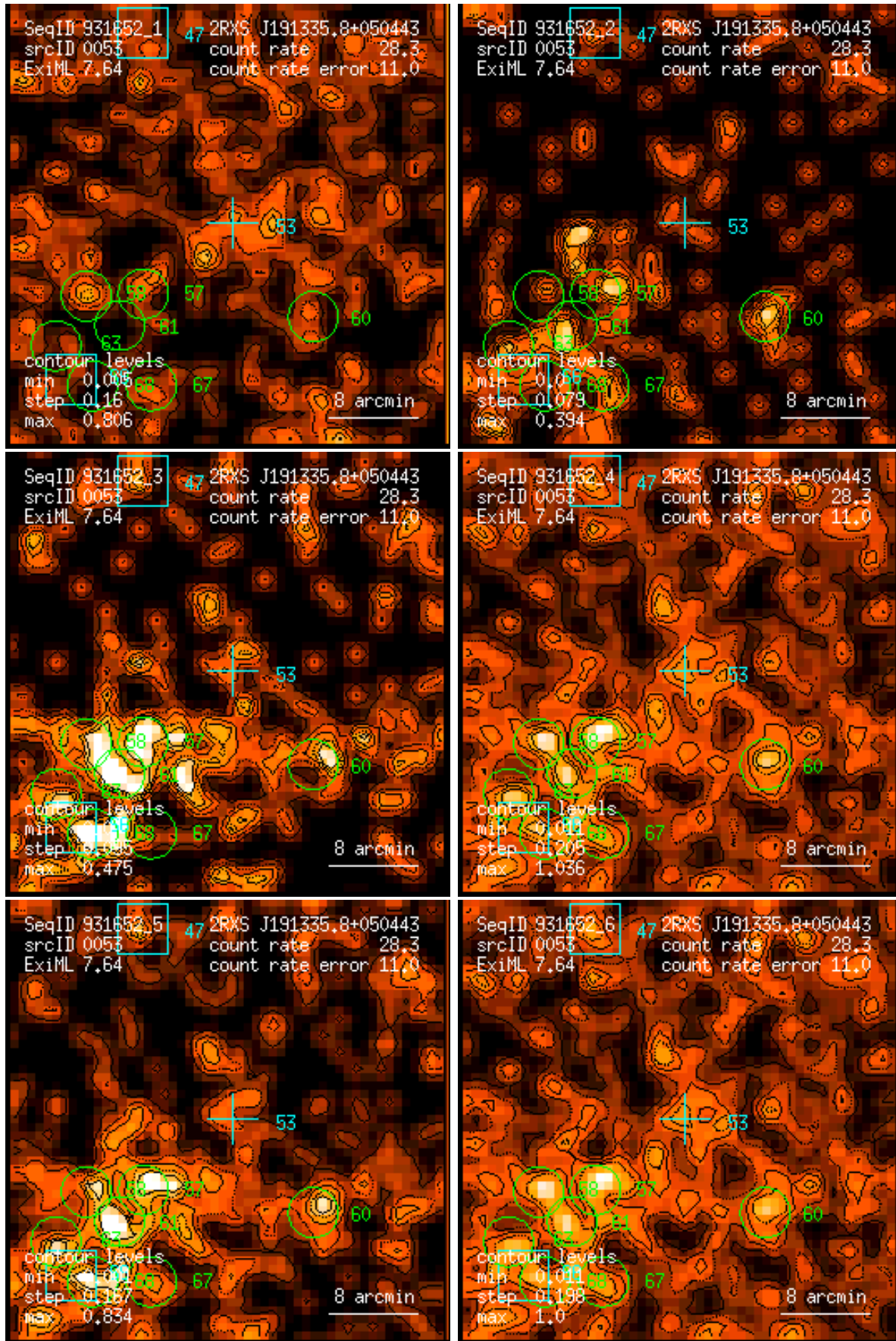
Figure 53: RASS 931652: detection 0053: band rate images, Gaussian filter: (1) PSPC channels 11 – 41, (2) 52 – 90, (3) 91 – 201, (4) 11 – 235, (5) 52 – 201, (6) 11 – 201. Broad band rates in counts/ks. Band rate contour levels in counts/ks/arcmin 2 .
