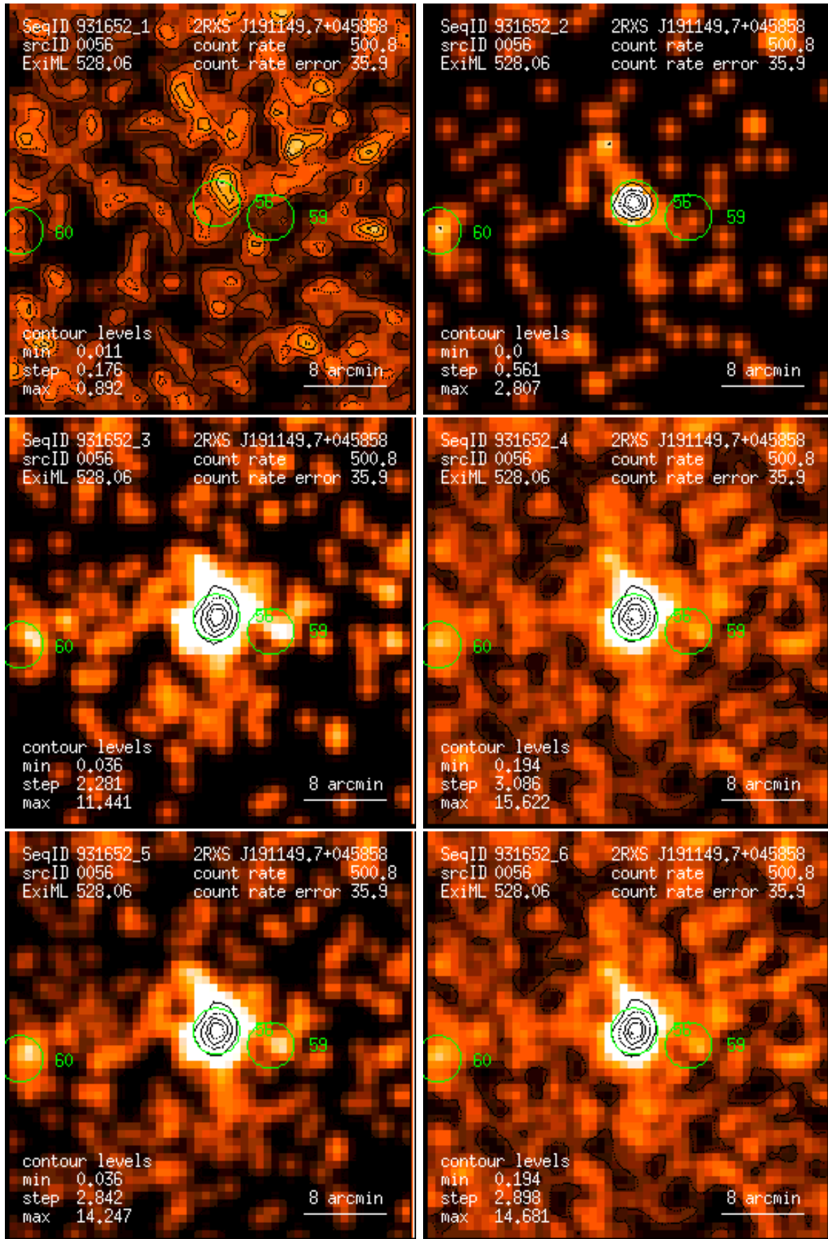
Figure 56: RASS 931652: detection 0056: band rate images, Gaussian filter: (1) PSPC channels 11 – 41, (2) 52 – 90, (3) 91 – 201, (4) 11 – 235, (5) 52 – 201, (6) 11 – 201. Broad band rates in counts/ks. Band rate contour levels in counts/ks/arcmin 2 .
