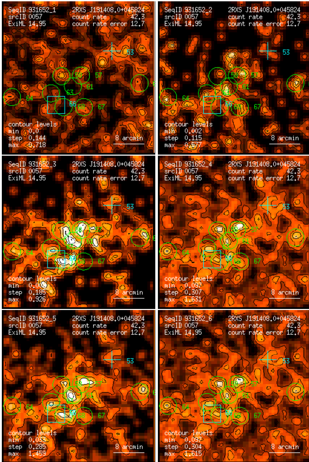
Figure 57: RASS 931652: detection 0057: band rate images, Gaussian filter: (1) PSPC channels 11 – 41, (2) 52 – 90, (3) 91 – 201, (4) 11 – 235, (5) 52 – 201, (6) 11 – 201. Broad band rates in counts/ks. Band rate contour levels in counts/ks/arcmin 2 .
