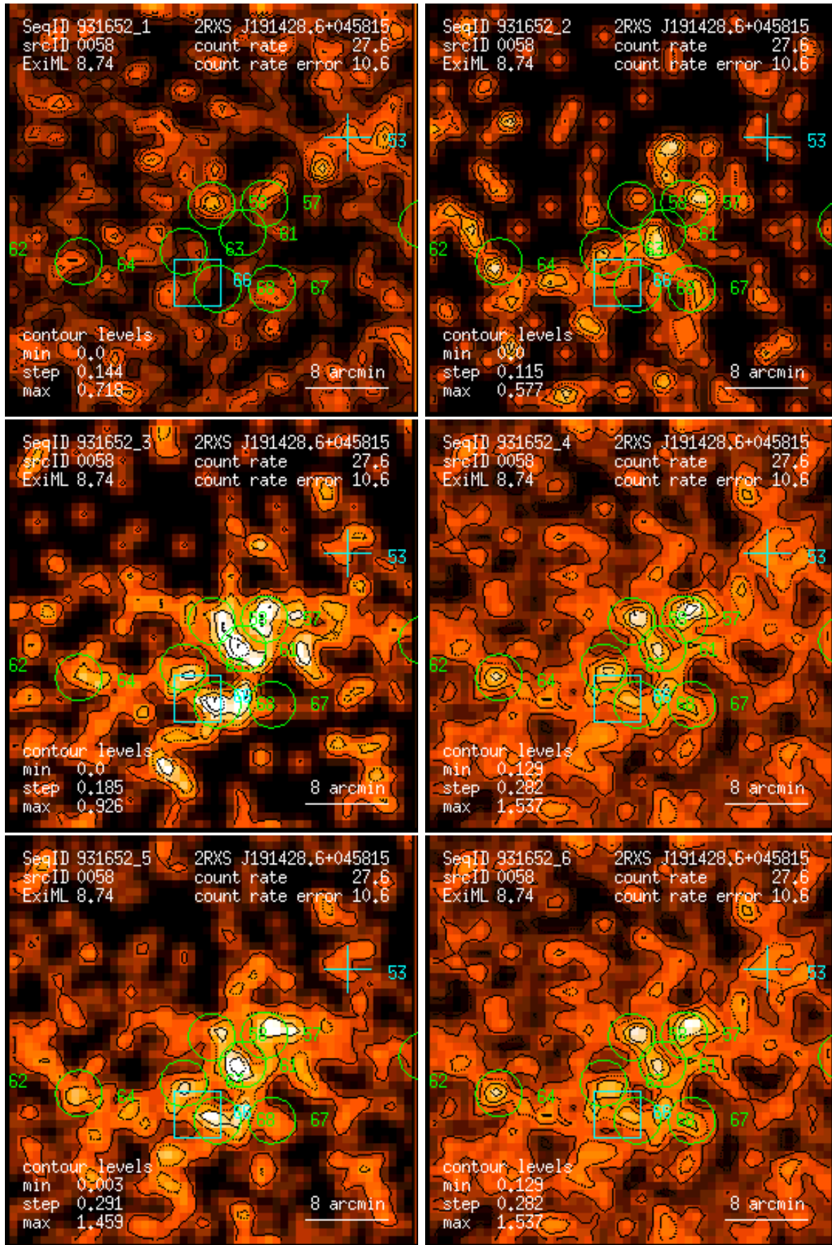
Figure 58: RASS 931652: detection 0058: band rate images, Gaussian filter: (1) PSPC channels 11 – 41, (2) 52 – 90, (3) 91 – 201, (4) 11 – 235, (5) 52 – 201, (6) 11 – 201. Broad band rates in counts/ks. Band rate contour levels in counts/ks/arcmin 2 .
