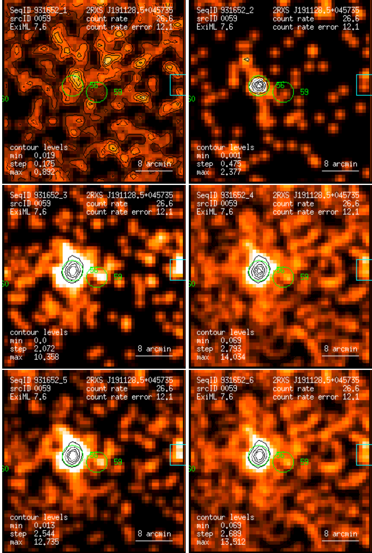
Figure 59: RASS 931652: detection 0059: band rate images, Gaussian filter: (1) PSPC channels 11 – 41, (2) 52 – 90, (3) 91 – 201, (4) 11 – 235, (5) 52 – 201, (6) 11 – 201. Broad band rates in counts/ks. Band rate contour levels in counts/ks/arcmin 2 .
