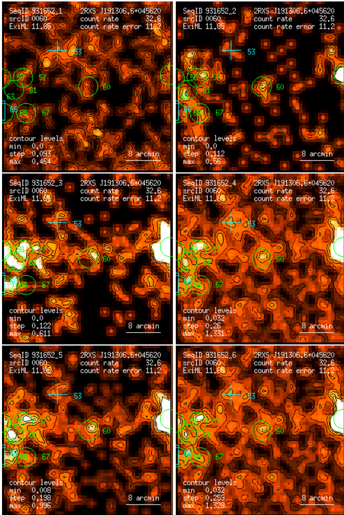
Figure 60: RASS 931652: detection 0060: band rate images, Gaussian filter: (1) PSPC channels 11 – 41, (2) 52 – 90, (3) 91 – 201, (4) 11 – 235, (5) 52 – 201, (6) 11 – 201. Broad band rates in counts/ks. Band rate contour levels in counts/ks/arcmin 2 .
